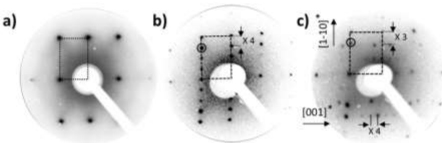
Figure 1: LEED patterns of (a) bare Ag(110) substrate, (b) after a deposition of \sim 1 ML of NaCl, (c) after the deposition of \sim 1 ML of silicon on NaCl/Ag(110). The Ag(110) unit cell, the x3 and x4 periodicities are indicated. The diffraction spot corresponding to NaCl film is highlighted by the small black circles in b and c. The LEED patterns were recorded at an energy of 70 eV.
