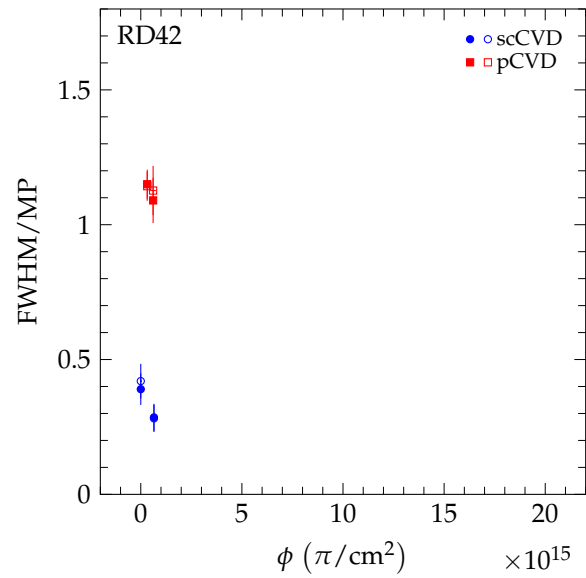
Figure 14. The FWHM/MP as a function of fluence in the pion irradiation measured in a +120 GeV/c hadron beam at CERN. The two values shown at each fluence are the values for positive (solid markers) and negative bias (open markers) at E = 2 \text{ V}/\mu\text{m} .
