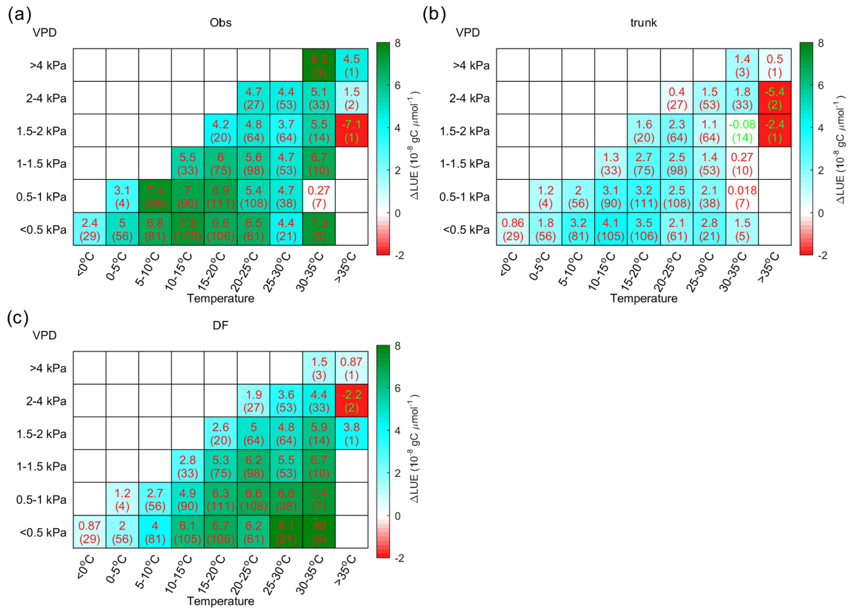
Figure 9. The distribution of the LUE difference between cloudy and sunny conditions ( \Delta LUE) in the temperature–VPD field. The upper numbers in each grid square indicate the average of the site-level \Delta LUE, while the numbers in parentheses indicate the number of sites with valid data. Panel (a) shows the \Delta LUE based on observations, panel (b) shows the \Delta LUE based on ORCHIDEE trunk, and panel (c) shows the \Delta LUE based on ORCHIDEE_DF.
