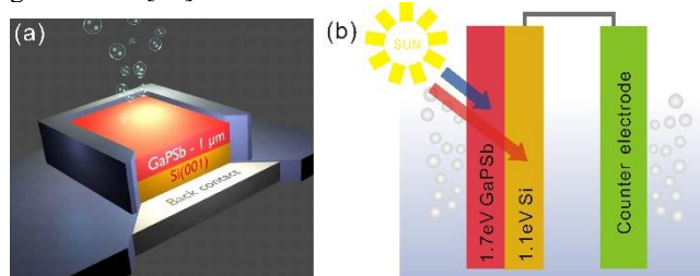
Fig. 1. (a) Schematic of the proposed GaP 1-x Sb x /Si tandem device for PEC water splitting. (b) Sunlight absorption illustration of GaP 1-x Sb x /Si tandem system with around 1.7/1.1eV bandgap combination for water splitting.
