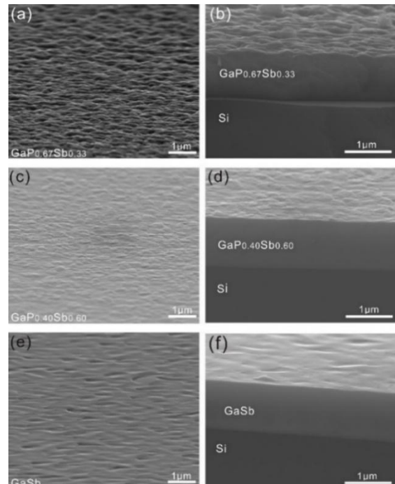
Fig. 3. Scanning electron microscopy (SEM) images of the \text{GaP}_{0.67}\text{Sb}_{0.33} , \text{GaP}_{0.40}\text{Sb}_{0.60} , \text{GaSb} three samples on plane view (a),(c),(e) and cross-section view(b),(d),(f).
