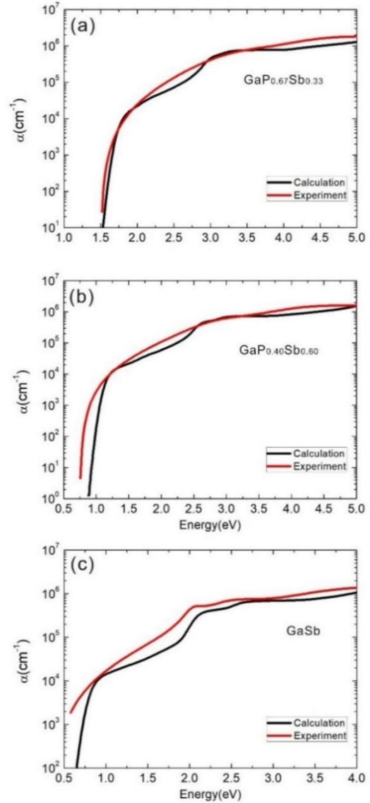
Fig. 4. Optical absorption spectra of the \text{GaP}_{0.67}\text{Sb}_{0.33} (a), \text{GaP}_{0.40}\text{Sb}_{0.60} (b), GaSb (c) semiconductors. The red lines were deduced from ellipsometry measurement and the black lines were obtained based on TB calculation.
