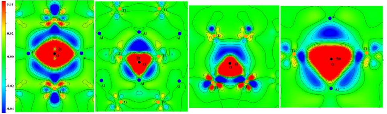
Figure 4. Charge transfer, \Delta\rho (in e/\text{\AA}^3 ), when sites are filled: oxygen in 2e (2D data displays in the [10 - 1] direction), 2h ( [-110] ), 4i ( [-100] ) and 4m ( [1 - 10] ) sites. Al atoms are in blue, Ti atoms in orange and O in black.
