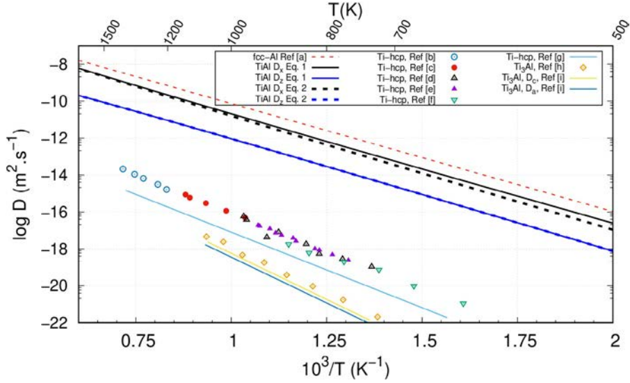
Figure 6. Diffusion coefficients of oxygen as a function of 1/T . Al: (a) = [29]; Ti-hcp: (b) = [30], (c) = [31], (d) = [32], (e) = [33], (f) = [34], (g) = [35]; \text{Ti}_3\text{Al} : (h) = [36]; (i) = [25].
