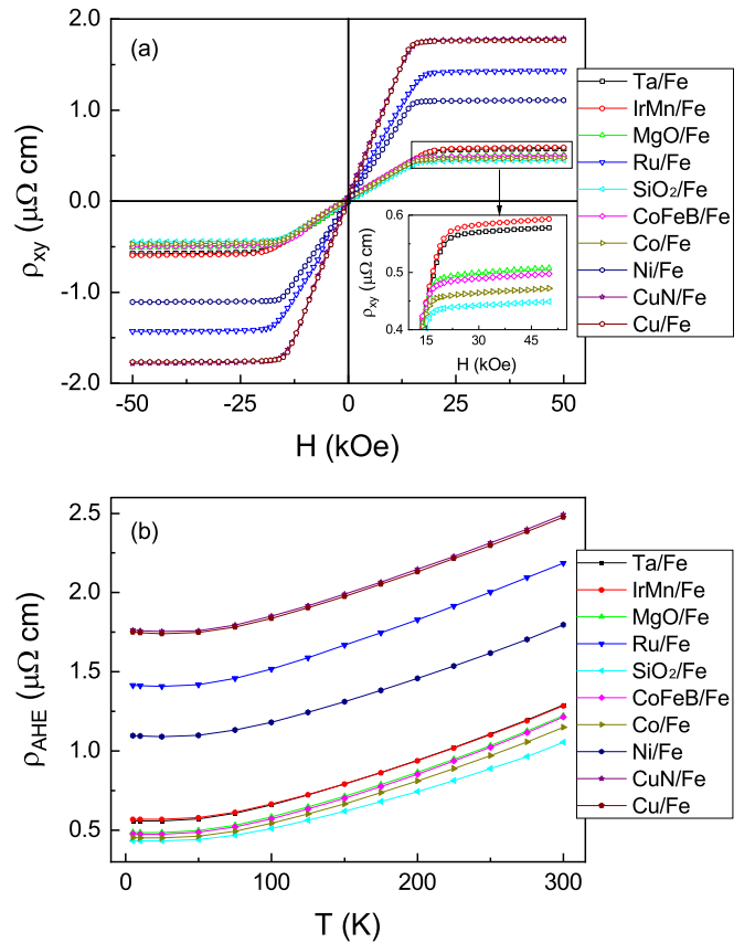
FIG. 3. (a) Field-dependent Hall resistivity ( \rho_{xy} ) of all samples measured at 5 K. (b) Temperature-dependent anomalous Hall resistivity ( \rho_{\text{AHE}} ) for all samples.
