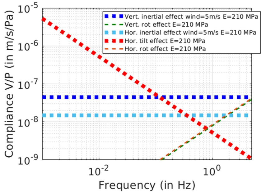
Figure 4. Theoretical prediction by Sorrells' theory of the ground Velocity over Pressure ratio ( V/P in m/s/Pa ) as a function of frequency (in Hz) for the vertical and horizontal components of ground velocity and for the three types of effects described in this section. Pressure perturbations are assumed to move horizontally with a wind speed of 5 m/s, and VBB sensor positions relative to SEIS center of mass given by Fayon et al. (2018) are taken into account.
