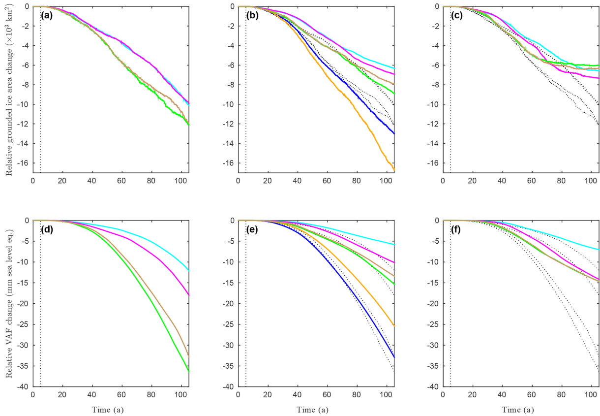
Figure 7. Evolution of grounded ice area in \times 10^3 km 2 (first row) and of volume above flotation in millimetre sea-level equivalent (second row) as a function of time during EXP_ABMB (coloured solid lines) relative to EXP_CONTROL for the inferred states I_{R_{y,\infty}} – panels (a) and (d), I_{R_{y,100}} – panels (b) and (e), and I_{R_{y,1}} – panels (c) and (f) – with the friction laws, linear Weertman (cyan), non-linear Weertman (magenta), Schoof with C_{\max} = 0.4 (green), Schoof with C_{\max} = 0.6 (brown), linear Budd (orange, for the inferred state I_{R_{y,100}} only) and non-linear Budd (blue, for the inferred state I_{R_{y,100}} only). The results obtained with the various friction laws for the inferred state I_{R_{y,\infty}} are reported on, respectively, (b–c) and (e–f) for ease of comparison (black dotted lines). The vertical black dotted lines mark the introduction of the perturbation at t = 5 a.
