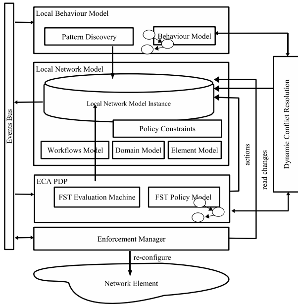
Fig. 3. Node Architecture
