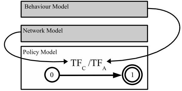
Fig. 6. Condition TF and Action TF are Computed using the Network Model and the Behaviour Model Respectively
