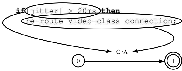
Fig. 4. Correspondence between if-then constituents and FST elements.
