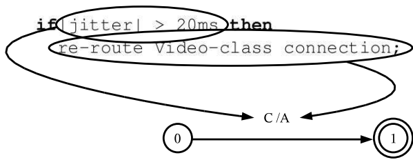
Fig. 4. Correspondence between if-then constituents and FST elements.
