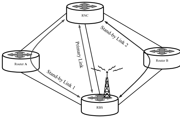
Fig. 7. Standby Link Scenario Network Schema
