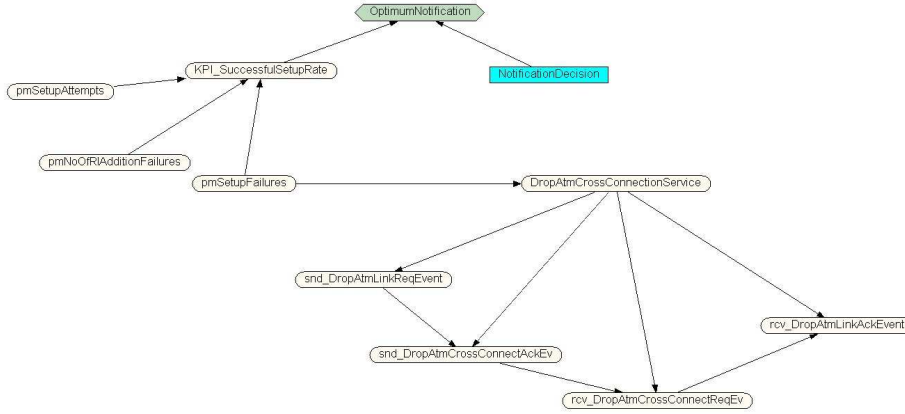
Fig. 5. Sample Bayesian Network composed of network event types
