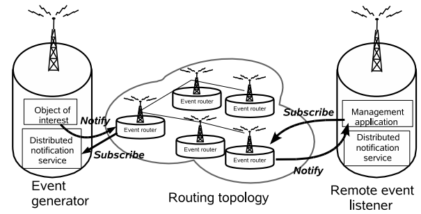
Fig. 1. Distributed Event Notification
