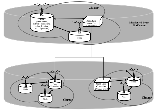
Fig. 2. Underlying Organisational Structure for Event Notification
