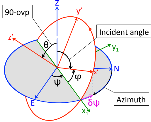
Figure 4. Sketch of the ellipse of polarization (red) with semi-major and semi-minor vectors x' and y' . The planarity vector z' is perpendicular to the ellipse plane. The geographical axes are E, N, Z and the Euler angles are \psi , \phi and \theta . The ellipse of polarization is defined by 3 angles: (1) the semi major vector azimuth with respect to North, (2) its incident angle with respect to the vertical and (3) the "out of vertical plane" (ovp) angle. The ovp angle is 0^\circ when the ellipse of polarization is in the vertical plane. The motion in the ellipse plane is from x' toward y' as indicated by the red arrow.
