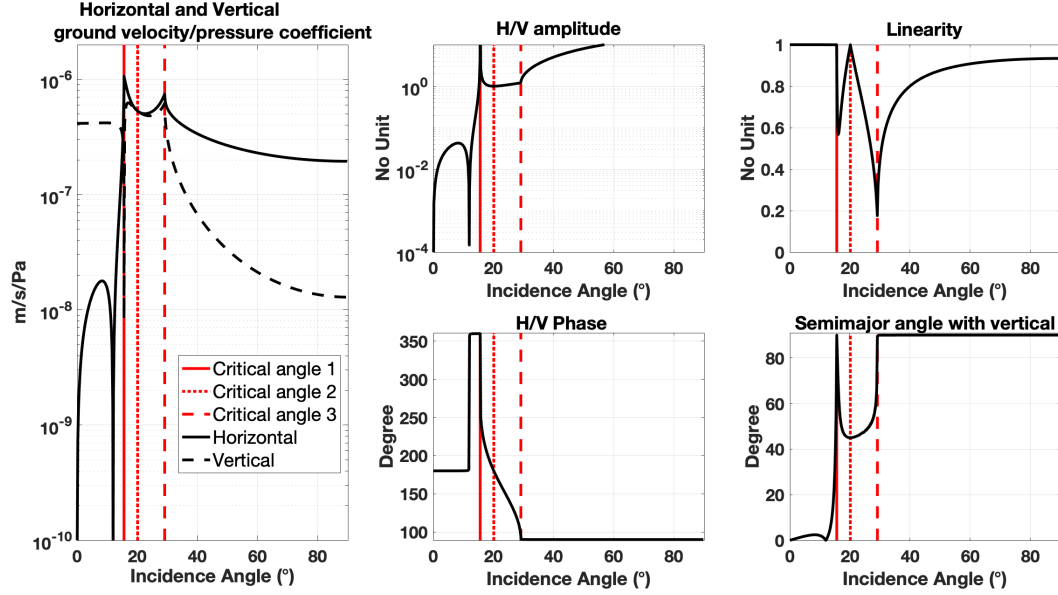
Figure 18. Transfer coefficient between the pressure amplitude of an acoustic wave and the horizontal and vertical ground velocity and impacts in terms of ground ellipticity. The left figure provides the transfer coefficient, as a function of incidence of the pressure wave with respect to vertical, between the amplitude of the pressure wave and the vertical and horizontal ground velocities for a simple interface between Mars’ atmosphere (with sound speed of 250 m/s and atmospheric density of 0.017 kg/m 3 ) and a brecciated bedrock (V p and V s of 926 m/s and 512 m/s respectively and density of 2600 kg/m 3 ). The two critical angles and the one canceling the P transmitted wave are detailed in the text and are shown by the three red lines (first critical angle related to P, angle for no P transmission and second critical angle related to S). The two middle figures show the amplitude and phase of the H/V ratio, as a function of incidence angle. Below the first critical angle of 15.6 degrees, the transfer coefficients are all real. They start to be complex after the first critical angle, with a variation from 360° to 90° of the H/V phase, until the second critical angle is reached, for an inclination of 29.1°. The phase remains to 90°. The last panel shows the linearity and the inclination of the semi-major axis of the elliptical signal. For linearity of 1, the semi-major axis is the axis of linear polarization. When the incidence angle increases from the first critical angle to the incidence cancelling transmitted P, the linearity decreases down to about 0.6 before reaching 1 again for an incidence angle of 20.1°. The angle of the semi-major axis varies from 90° to 45° with respect to vertical. The same type of variation occurs between the 20.1° incidence and the second critical angle, with the linearity decreasing down to about 0.2 for the third critical angle and again a rotation of the semi-major axis. The semi-major axis remains vertically oriented after the second critical angle, while the linearity is growing toward 1 for large incidences.
