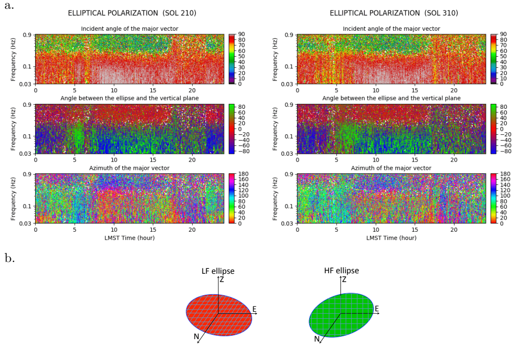
Figure 7. For signals with elliptical polarization, incident angle of the major axis (a. top), angle between the ellipse and the vertical plane (a. middle) and azimuth of the major vector (a. bottom) as a function of LMST time and frequency for sol 210 (a. left) and 310 (a. right). Angles are all in degrees. Azimuth are between 0 and 180^\circ with an ambiguity of 180^\circ . A sketch of the high frequency and low frequency ellipse of polarization is shown in b.
