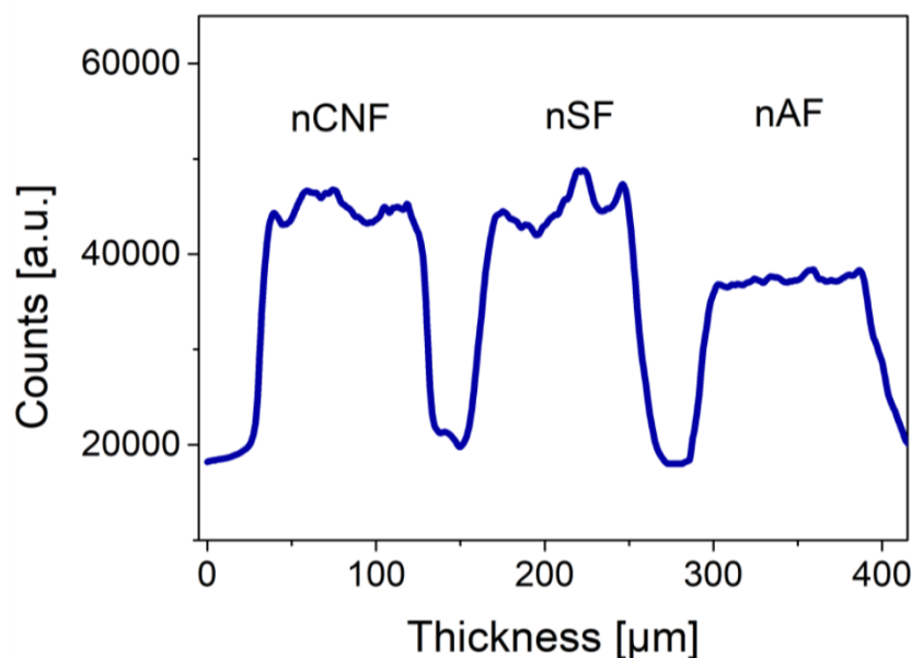
Figure 6. Cross section in z-direction from the \mu -CT data analysis from sheets containing nanoparticle labeled particles taking the entire signal of an area of 500 \mu\text{m} \times 500 \mu\text{m} in width into account. The wire side is left for nCNF, and right for nSF and AF.
