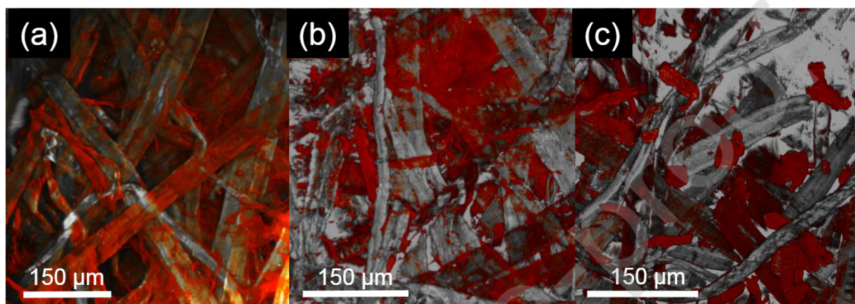
Figure 3. Multiphoton microscopy images highlighting (a) fCNF (b) fSF and (c) fAF added to the sheet at 10 wt%. Pulp fibers are depicted in grey while the fluorescent labeled samples are red.
