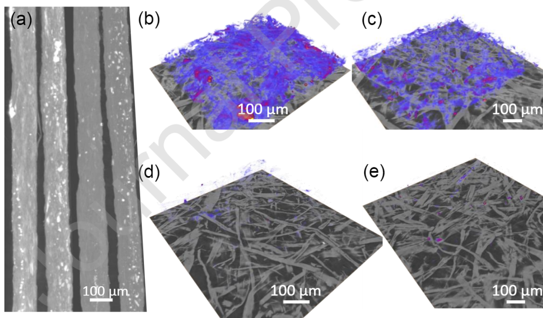
Figure 5. X-ray microtomography data showing (a) the cross section of the paper stack (nCNF, nSF, nAF and CNF, from left to right) and the distribution of (b) cellulose nanofibrils, (c) secondary fines and (d) ARBOCEL® fiber fragments compared to a (e) blank containing 10% untreated CNF.
