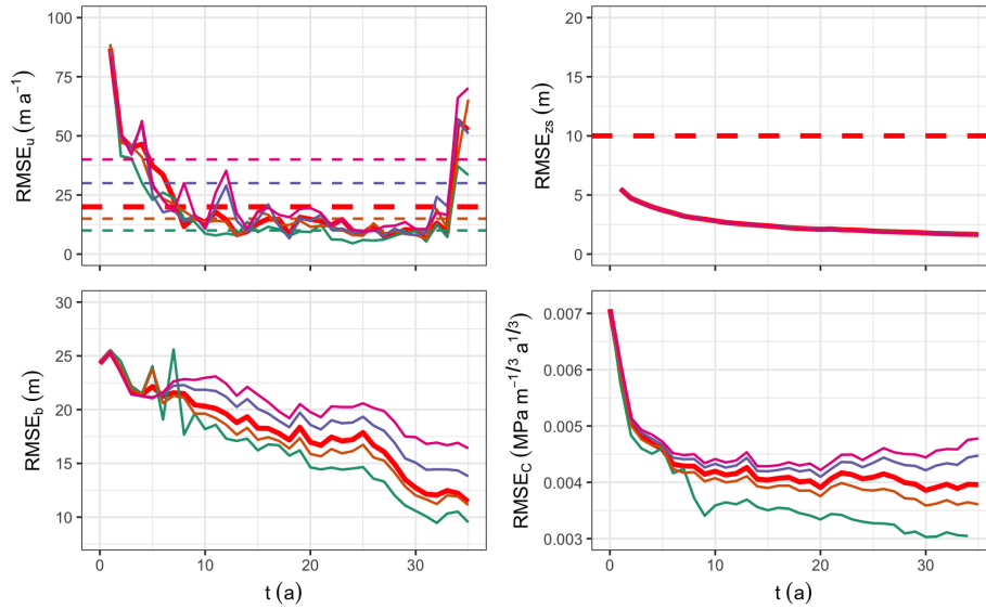
Figure 10. Sensitivity to the surface velocity observation error \sigma_u^{obs} : RMSEs after each analysis, computed only for x \geq 300 km for b and C . The thick red lines correspond to the results with \sigma_u^{obs} = 20 \text{ m a}^{-1} and \sigma_{z_s} = 10 \text{ m} shown in Figs. 3 and 9. The horizontal dashed lines correspond to the observation errors \sigma_u^{obs} and the results are presented with solid lines using the same colour code. \sigma_{z_s}^{obs} = 10 \text{ m} for all the experiments.
