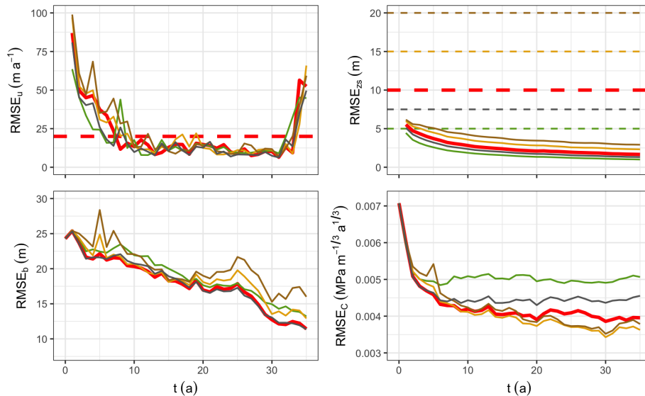
Figure 11. Sensitivity to the surface elevation observation error \sigma_{z_s}^{obs} : RMSEs after each analysis, computed only for x \geq 300 km for b and C . The thick red lines correspond to the results with \sigma_u^{obs} = 20 \text{ m a}^{-1} and \sigma_{z_s} = 10 \text{ m} shown in Figs. 3 and 9. The horizontal dashed lines correspond to the observation errors \sigma_{z_s}^{obs} and the results are presented with solid lines using the same colour code. \sigma_u^{obs} = 20 \text{ m a}^{-1} for all the experiments.
