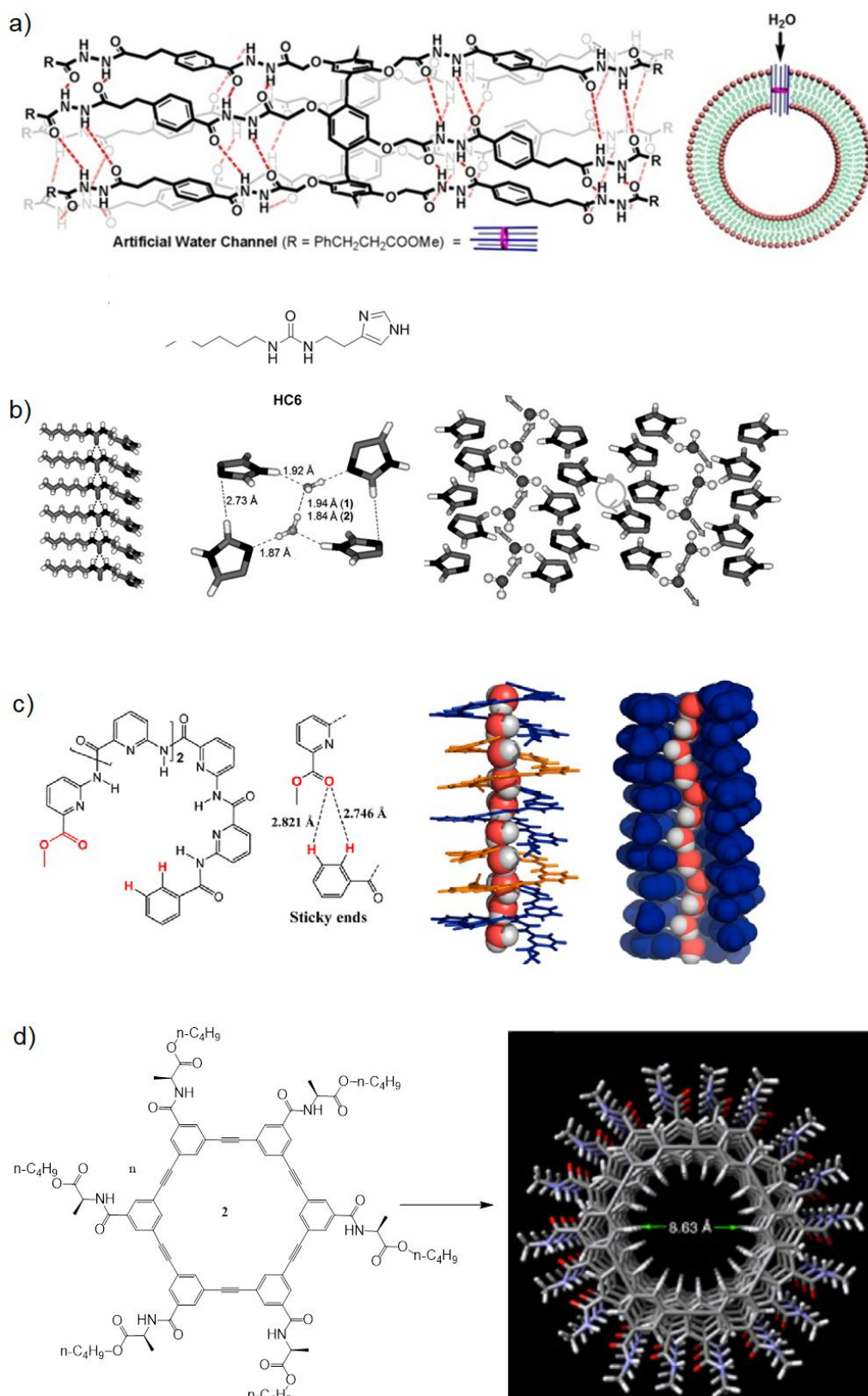
Figure 4. a) Single molecular PAP1 water channels [43]; b) Single crystal structure of hexyl-ureidoethylimidazole and its related urea H-bonding ribbons and of I-quartets that present d) dipolar orientation of water [34]; c) X-ray single crystal structure and d) representation of a single water file Aquafoldamers [48] d) Simulated structure of macrocyclic channels [49]. (image adapted with permissions from reference [34,43,48,49])
