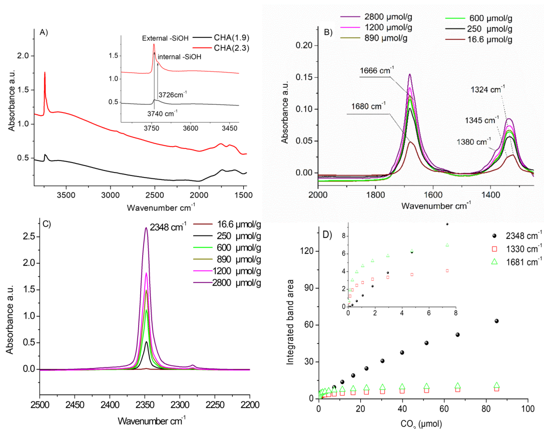
Figure 4. IR spectra of CHA(1.9) and CHA(2.3) after activation at 350 °C under vacuum in the region 1500-4000 cm -1 (the spectra were normalized to 20 mg (A)). IR spectra under pulsed CO 2 adsorption on CHA(2.3) in the regions of 2000-1250 cm -1 (B), 2500-2200 cm -1 (C) and integrated area of bands in FTIR spectra corresponding to chemisorbed CO 2 at 1330 cm -1 and 1681 cm -1 and physisorbed CO 2 at 2348 cm -1 ; (D)
