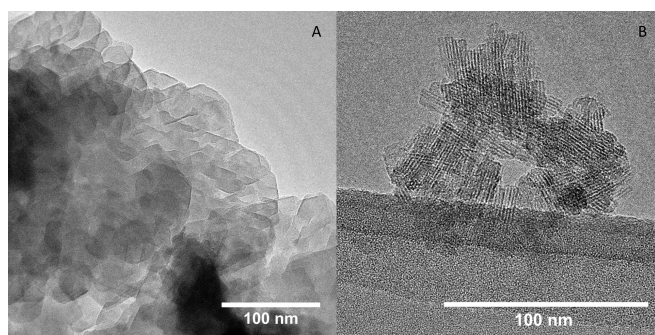
Figure 2. TEM images of samples CHA(1.9) (A) and CHA(2.3) (B).
