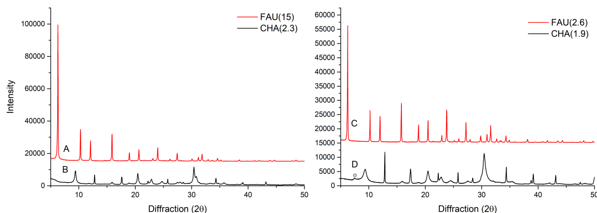
Figure 1. XRPD patterns of (A) FAU(15), (B) CHA(2.3), (C) FAU(2.6), and (D) CHA(1.9); trace of impurity marked with circle.
