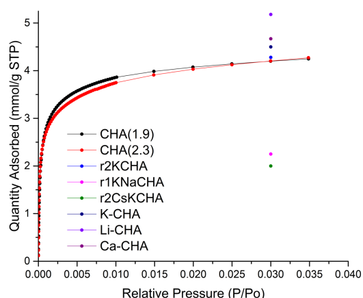
Figure 3. CO 2 adsorption of samples CHA(2.3) (red) and CHA(1.9) (black) at 273.15 K. CO 2 capacity from Zhang et al. 7 (K-CHA, Li-CHA, and Ca-CHA) and Shang et al. 12 (r1KNaCHA, r2KCHA, and r2CsKCHA) reported as single points at relative pressure of 0.030 (104 kPa).
