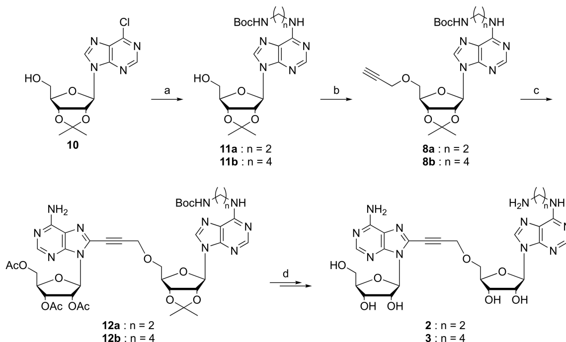
Scheme 1. Reagents and conditions: (a) \text{BocNH}(\text{CH}_2)_n\text{NH}_2 , DME, \text{NEt}_3 , 80 °C, 66% ( n = 2 ) or 91% ( n = 4 ); (b) NaH, propargylbromide, THF, 4 °C, 60% or 68%; (c) 6, \text{Pd}(\text{PPh}_3)_4 , CuI, \text{NEt}_3 , THF, 60 °C, 37% or 40%; (d) 28% \text{NH}_4\text{OH}/\text{MeOH} , rt; TFA/ \text{H}_2\text{O} , 4 °C, 42% or 61% in two steps.
