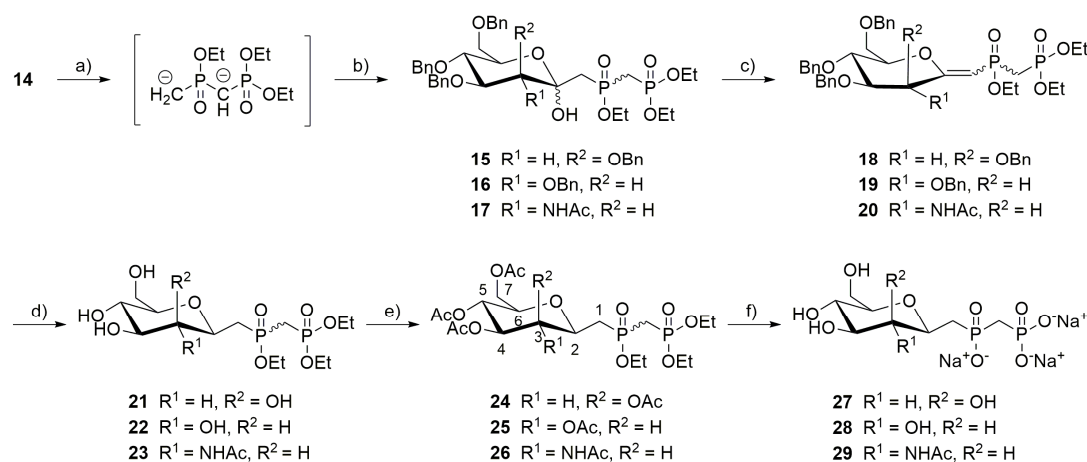
Scheme 3. Reagents and conditions: (a) n BuLi, THF, -78\text{ }^{\circ}\text{C} , 1 h. (b) 11 , 12 or 13 , THF, -78\text{ }^{\circ}\text{C} , 2 h, 58% for 15 , 58% for 16 , 25% for 17 . (c) (\text{CF}_3\text{CO})_2\text{O} , pyridine, \text{CH}_2\text{Cl}_2 , 0\text{ }^{\circ}\text{C} , 3 h, 80% for 18 , 70% for 19 , 63% for 20 . (d) \text{H}_2 , Pd/C 10%, EtOH, RT, 16 h. (e) \text{Ac}_2\text{O} , pyridine, 80% for 24 , 96% for 25 , 73% for 26 . (f) i. TMSBr, \text{CH}_2\text{Cl}_2 , 0\text{ }^{\circ}\text{C} to RT, 16h; ii. NaOH, \text{H}_2\text{O} , RT, 16 h, 95% for 27 , 92% for 28 , 85% for 29 .
