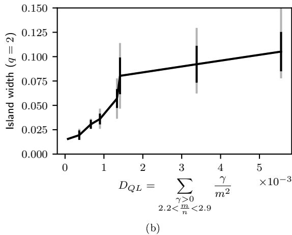
FIG. 9: Island size on q = 2 surface, as a function of input power (a), and as a function of a quasilinear estimate of the turbulent heat diffusivity D_{QL} (b). The black errorbars correspond to the standard deviation during the last 5000\tau_A of the simulation ; the grey bars represent the min/max values.
