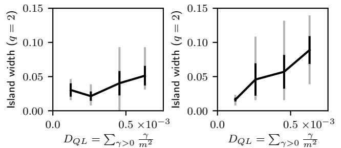
FIG. 10: Island size on q = 2 surface, as a function of quasilinear estimate of the turbulence level, without (left) and with (right) a source maintaining the initial pressure profile. Those simulations are performed in cylindrical geometry, with parameters matching previous work 14 .
