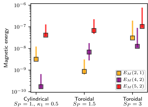
FIG. 6: Magnetic energy at saturation of the most important modes, in cylindrical and toroidal simulations.
