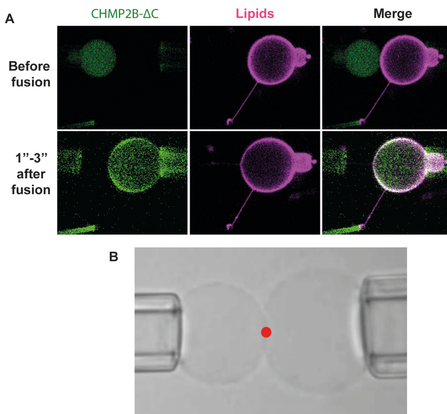
Figure 4. Positioning and fusion of GUVs. A. Fluorescent image of GUVs before and immediately after fusion. Lipid mixing is still not completed. The contrast in the image after fusion has been enhanced to show that fusion occurs without protein leaking outside the GUVs. Scale bar = 10 \mu M. B. DIC imaging of GUVs optimal position before fusion. The red dot indicates the position of the optical tweezers. Scale bar = 10 \mu M.
