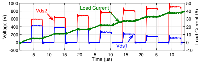
Fig. 12. Experimental results. Voltage unbalancing across two series-connected SiC-MOSFETs; classical planar package.
