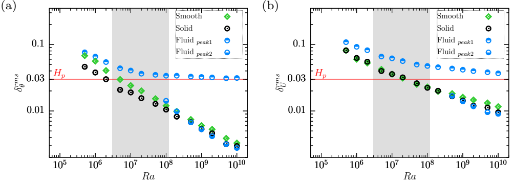
FIGURE 10. RMS-based boundary layer thicknesses as a function of Ra and for each space-averaging zone (smooth, solid and fluid). See equations 5.1 and 5.2 for definitions. (a) Thermal boundary layer thickness \delta_\theta^{rms} measured as the peak of \theta_{rms} ; (b) kinetic BL thickness measured as the peak of U_{rms} . The shaded area illustrates the Ra -range of the regime II. The red line marks the roughness height ( H_p ).
