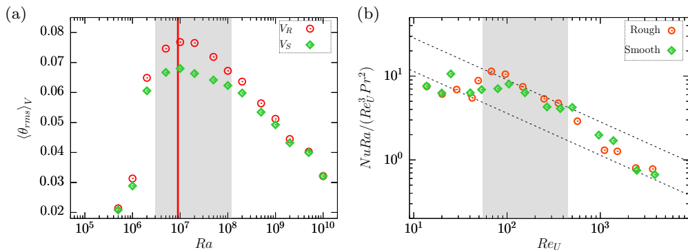
FIGURE 13. (a) Integral of rms temperature fields over the fluid volume of a half cavity ( V_R volume of the rough half cavity ; V_S volume of the smooth half cavity). The vertical red line represents the critical Rayleigh number Ra_c . (b) Friction coefficient normalized by dissipation vs Reynolds number. The dashed lines display Re_U^{-0.5} power laws.
