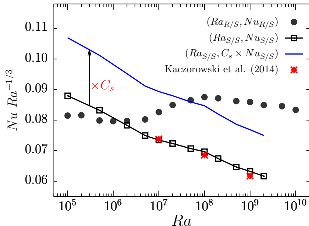
FIGURE 2. Compensated Nusselt number as a function of Rayleigh number for the fully smooth cavity ( S/S ) and the asymmetric cavity ( R/S ). The blue line corresponds to the increased Nusselt number by a factor corresponding to the relative increase of the heat exchange surface in the ( R/S ) cavity. Red points refer to DNS results from Kaczorowski et al. (2014) .
