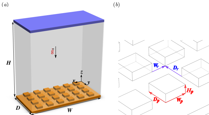
FIGURE 1. (a) Asymmetric Rayleigh-Bénard cavity ( R/S ) with a rough bottom plate. (b) Blow-up of the spatial arrangement of the blocks regularly distributed.
