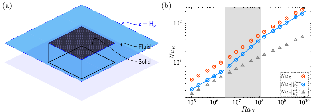
FIGURE 5. (a) Sketch of the geometric division of the horizontal plane at z = H_p . (b) Separation of rough heat flux at z = H_p ( Nu_R|_{H_p} ) into contribution from the fluid interface ( Nu_R|_{H_p}^{fluid} ) and from the solid surface ( Nu_R|_{H_p}^{solid} ). The solid lines correspond to the least-squares fits of the results on the fluid interface for the three regimes: regime I: Nu_R|_{H_p}^{fluid} \sim 0.041Ra_R^{0.34} , regime II: Nu_R|_{H_p}^{fluid} \sim 0.005Ra_R^{0.49} and regime III: Nu_R|_{H_p}^{fluid} \sim 0.072Ra_R^{0.34} . The shaded area marks the Ra -range of the heat transfer regime II.
