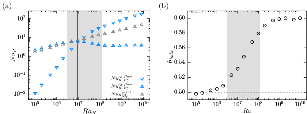
FIGURE 6. (a) Comparison of the different contributions from the solid surface Nu_R^{solid|fluid} and the fluid interface ( Nu_R^{cd|fluid} and Nu_R^{cv|fluid} ) to the rough heat flux Nu_R at z = H_p as a function of the rough Rayleigh number ( Ra_R ). The vertical red line marks the critical Rayleigh number ( Ra_c ). (b) Bulk temperature ( \theta_{bulk} ) as a function of Ra_R . The shaded area marks the Ra -range of the heat transfer regime II.
