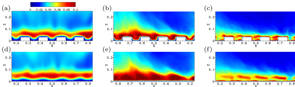
FIGURE 11. Temperature fluctuation rms field ( \theta_{rms} ) on vertical planes close to the rough plate for three particular Ra : (a,d) Ra = 2 \cdot 10^6 (regime I) ; (b,e) Ra = 5 \cdot 10^7 (regime II) ; (c,f) Ra = 10^9 (regime III). (a,b,c) between two rows of roughness blocks y = 0.3125 , (d,e,f) at mid-depth of the cavity y = 0.25 ).
