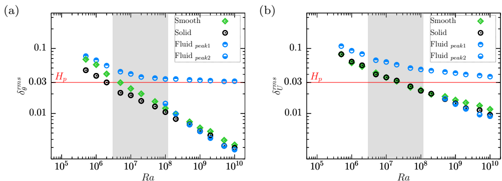
FIGURE 10. RMS-based boundary layer thicknesses as function of Rayleigh number Ra and of the space-averaging zone (smooth, solid and fluid), see equations 5.1 and 5.2 for definition. (a) Thermal BL thickness \delta_\theta^{rms} measured as the peak of \theta_{rms} ; (b) kinetic BL thickness measured as the peak of U_{rms} . The red line marks the roughness height ( H_p ).
