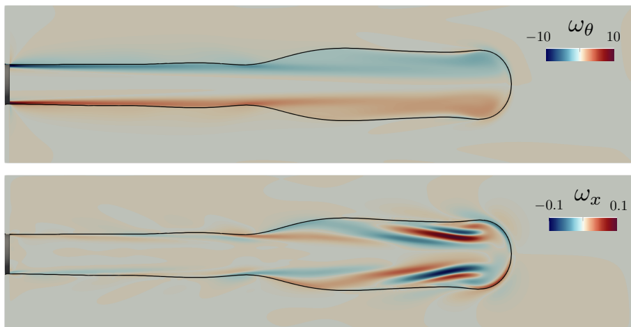
Figure 3: Two-dimensional representation of the interfacial location together with \omega_\theta (top panel) and \omega_x (bottom panel) in the x - z plane ( y = 2 ) for Case 1 in table 2 ( Re = 1000 and We = 30 ) at t = 24.38 . The colour represents the respective vorticity field, where appropriate scales are shown in each panel.
