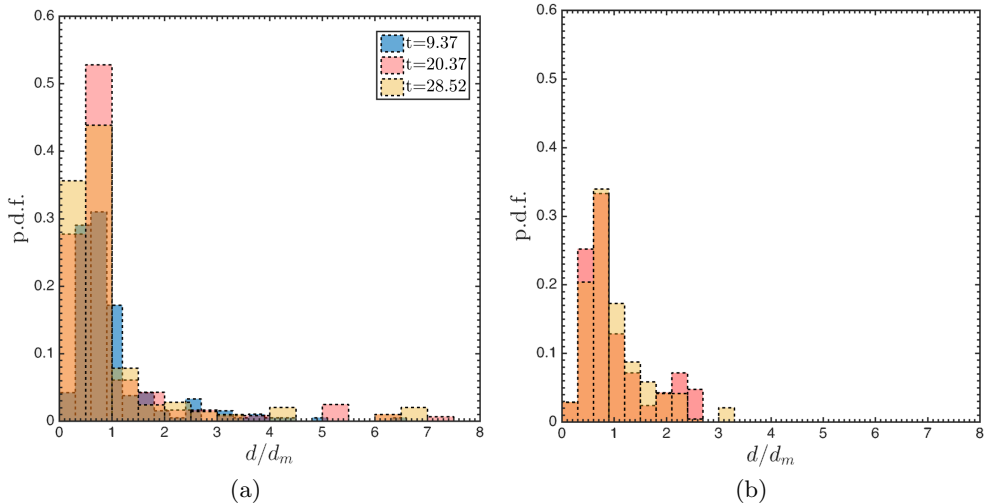
Figure 13: Probability density function (p.d.f.) for the entrapped and injected droplets for Case 4 ( Re = 6530 and We = 303 ) at t = 9.37 , 20.37 , and 28.52 shown in panels (a) and (b), respectively. The distributions are normalised by the calculated mean diameter for each time, d_m .
