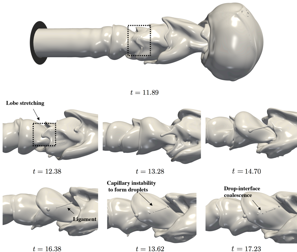
Figure 10: Three-dimensional representation of the interface showing the spatio-temporal evolution of the formation of droplets via the stretching of the outer lobe for Case 4 ( Re = 6530 and We = 303 ). Dimensionless times are shown in each panel.
