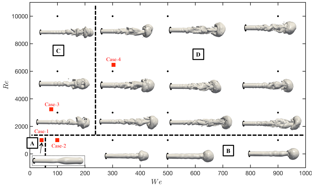
Figure 2: Regime map of the phenomenological interfacial dynamics in the Re - We space using the M2 -mesh (see table 4 in Appendix for mesh details). Four different regimes and their boundaries are identified. A snapshot of the flow corresponding to the three-dimensional representation of the interface for each simulated point (i.e., black marker) is shown. The red squares refer to the cases presented in table 2.
