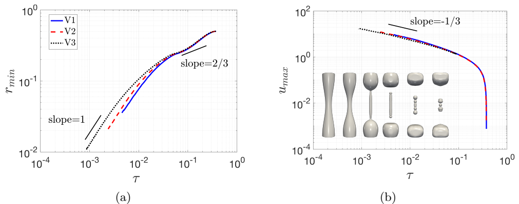
Figure 15: Scaling laws for the capillary singularity of a water-thread surrounded by air for different numerical resolutions (see table 5). Here, the Ohnesorge number is 1.178 \times 10^{-3} . The minimum thread radius, (a), and the maximum streamwise velocity, (b), versus the remaining time to breakup \tau , agree with the inertial-capillary and inertial-viscous regimes presented by Eggers (1993); Day et al. (1998). Additionally, a three-dimensional representation of the interface is shown to depict the retraction of the satellite ligament to produce daughter droplets via the ‘end-pinching’ mechanism (in agreement with Notz & Basaran (2004)).
