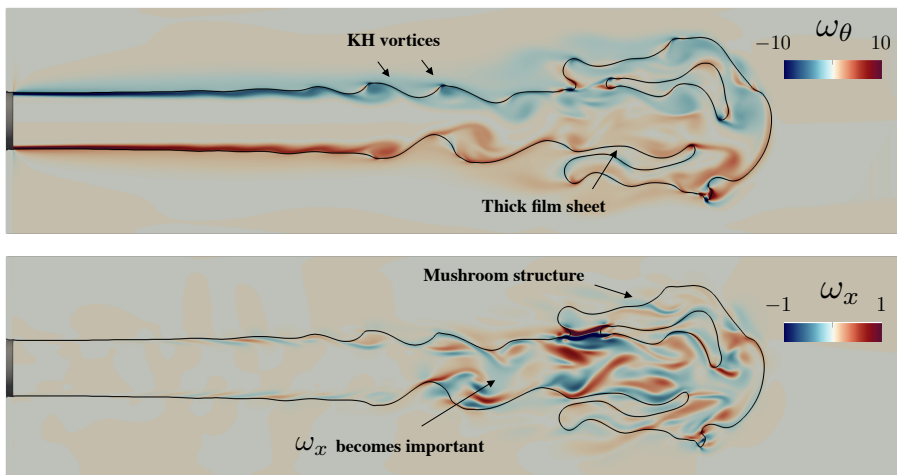
Figure 5: Two-dimensional representation of the interfacial location together with \omega_\theta (top panel) and \omega_x (bottom panel) in the x-z plane ( y=2 ) for Case 3 in table 2 ( Re=3260 and We=75 ) at t=24.65 . The colour represents the respective vorticity fields, where appropriate scales are shown in each panel.
