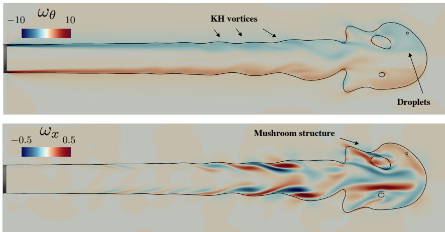
Figure 4: Two-dimensional representation of the interfacial location together with \omega_\theta (top panel) and \omega_x (bottom panel) in the x-z plane ( y=2 ) for Case 2 in table 2 ( Re=1000 and We=100 ) at t=26.87 . The colour represents the respective vorticity fields, where appropriate scales are shown in each panel.
