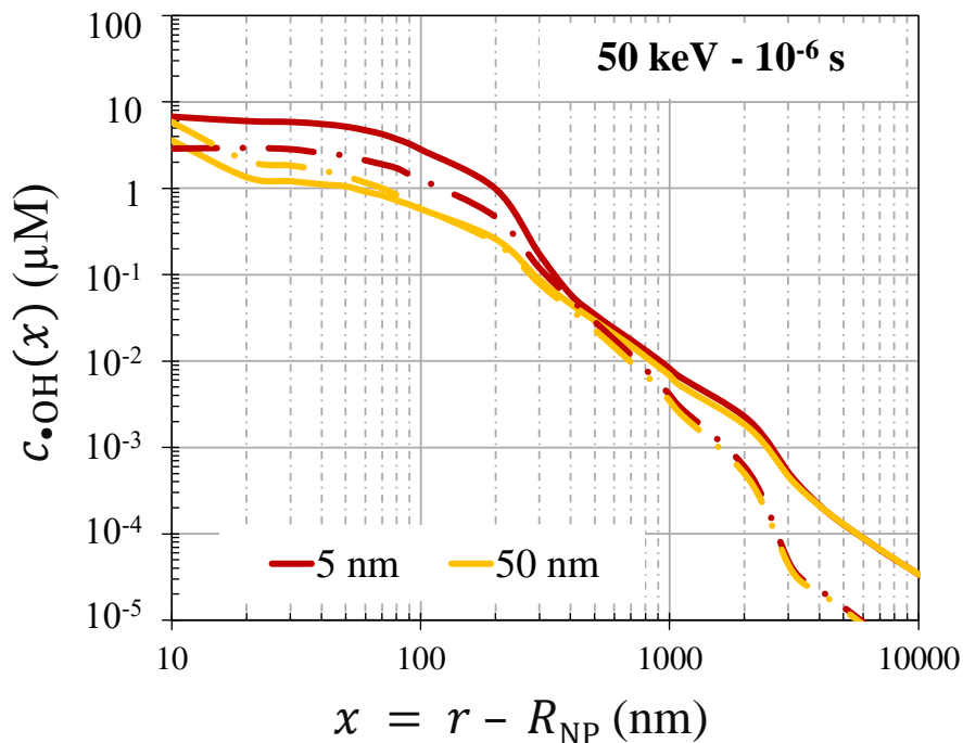
Figure 2: Radial concentration c_{\bullet OH}(x) as a function of x ( E_{\text{photon}} = 50 keV and t = 10^{-6} ), for two R_{\text{NP}} . Solid line shows results for a GNP and dashed line for a WNP.
