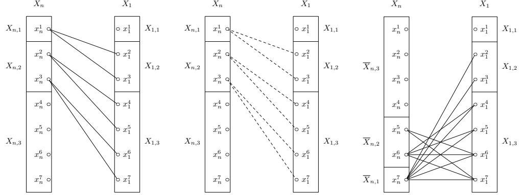
Figure 2: An expanding matching, an expanding antimatching and an expanding crossing
