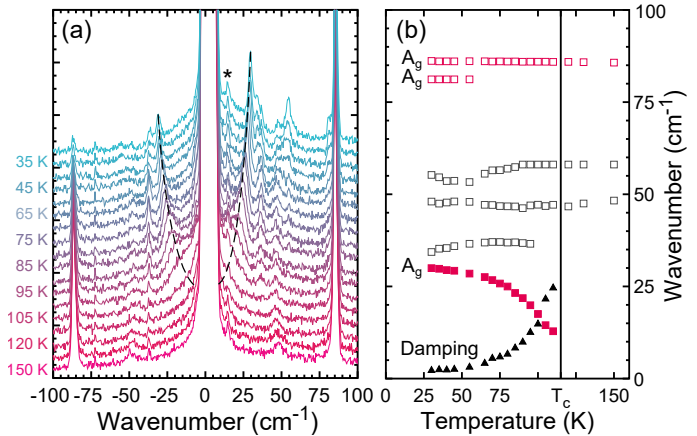
Figure 2. (a) Low-frequency Stokes–Anti-Stokes Raman spectra as a function of temperature across the phase transition. The dashed line is a guide to the eye for the behavior of the soft mode. The peak marked with an asterisk * is an artefact. (b) Mode frequencies as a function of temperature. The soft-mode data are pictured with full symbols, including its damping shown as black triangles.
