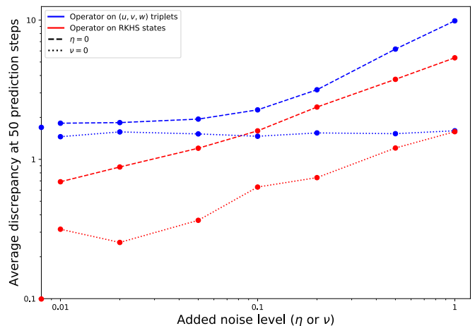
FIG. 9. Sensitivity when predicting trajectories along the Lorenz-63 attractor: Reconstruction error dependency on noise levels. Data for the \nu = \eta = 0 noiseless case is shown as markers on the vertical axis.
