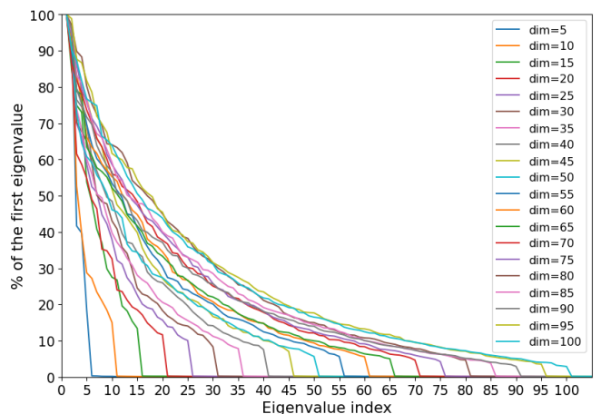
FIG. 10. Eigenvalues for the reconstruction of Lorenz-96 attractor, randomly projected in dimension 1000, with added high-dimensional noise, for N = 10000 samples. The dimension in the legend refers to the original parametrization of Lorenz-96 attractor, which is recovered by the algorithm in the form of a spectral gap when reconstructed from the 1000-dimensional noisy time series. Values after the gap are very low and given in Table I, together with the gap itself.
