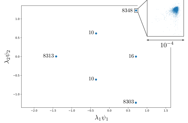
FIG. 5. Projection of the mess3's causal states on the reduced basis \{\Phi_1, \Phi_2\} . The number of samples stacked on each point is indicated.
