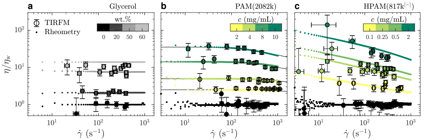
Figure 3: Comparison of the mechanical behaviours of: (a) water/glycerol mixtures; (b) PAM(2082k) solutions; and (c) HPAM(817k [−1] ) solutions. TIRFM velocimetry data are plotted in circles and rotational rheometry data are plotted using dots; black lines in panel (b) indicate predictions of the universal model of Ref. [34]. The color bars indicate the concentration of each solution and water is always represented in black. All the data shown here were collected without added salt.
