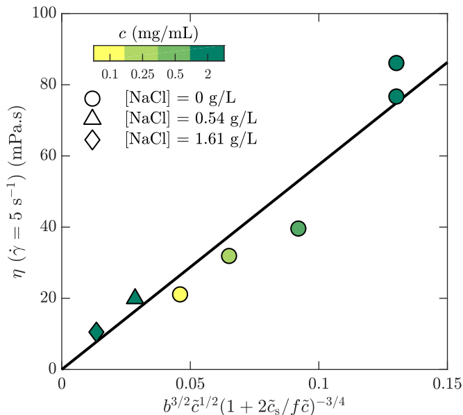
Figure 7: Bulk rheology measurements of the steady-shear viscosity for HPAM(817k [−] ) at a shear rate of 5 s −1 , as a function of the scaling variable developed by Dobrynin and coworkers. [41]
