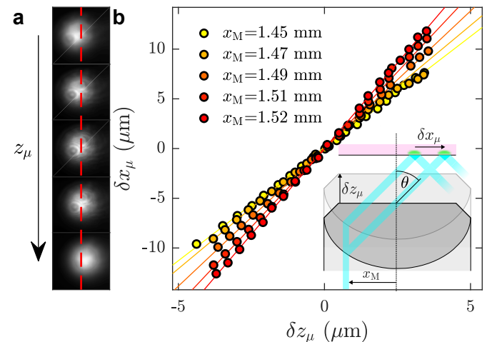
Figure 6: Incident angle calibration. (a) Raw images of the laser beam spot for the in situ calibration. Successive images show the spot shifting as imposed z_\mu increases. The red dashed line represents the position of the spot when \delta z_\mu = 0 . (b) Measured spot position \delta x_\mu as a function of z_\mu for different values of x_M . Straight lines display linear fits of the data.
