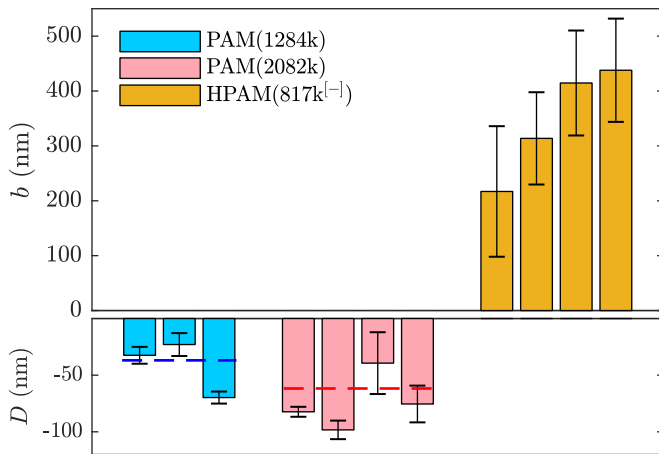
Figure 4: Comparison slip length for different PAM and HPAM solutions as an average over all imposed pressures, each bar corresponding to a different concentration. From left to right: for PAM(1284k) the concentrations are c = \{4, 12, 20\} \text{ mg mL}^{-1} ; for PAM(2082k), c = \{2, 4, 8, 10\} \text{ mg mL}^{-1} ; and for HPAM(817k [-1] ), c = \{0.1, 0.25, 0.5, 2\} \text{ mg mL}^{-1} . The dashed lines in the bottom panel indicate the mean over all concentrations for the associated molar mass.
