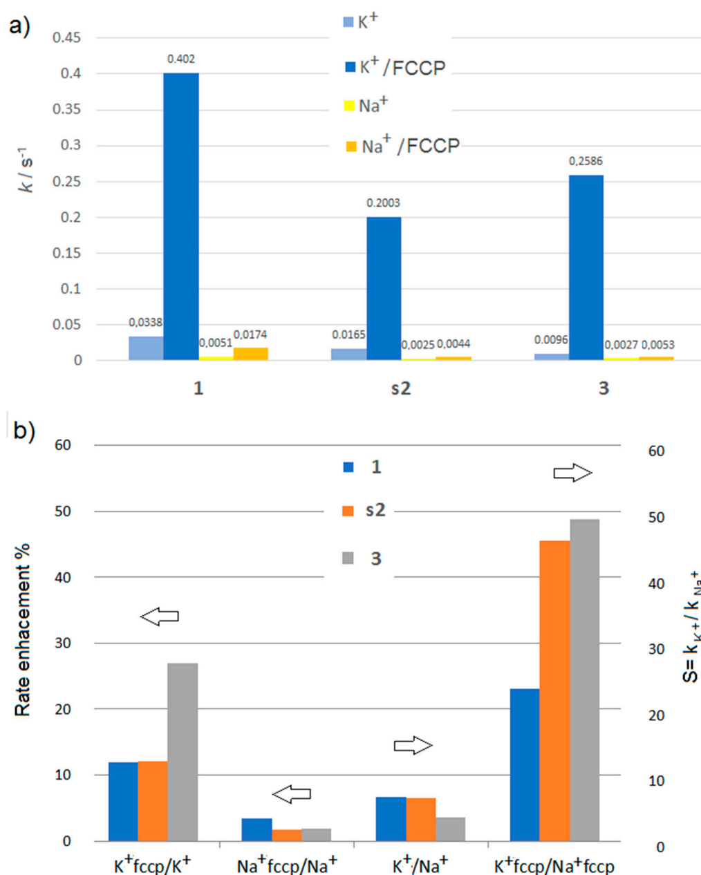
Figure 4. Bar graphs showing (a) the pseudo-first-order rate constants k (s -1 ) for the transport of K + and Na + cations and (b) rate enhancement and K + /Na + selectivity, for the macrocyclic carriers 1 , s2 , 3 , (12.9 mol%) in presence or absence of protogenic FCCP carrier.
