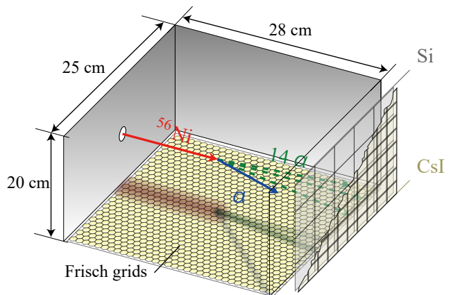
Fig. 1. (Color online) Schematic view of the experimental setup with the MAYA detector. A ^{56}\text{Ni} beam (red) enters the active volume of MAYA and interacts with the helium gas resulting in the excitation of ^{56}\text{Ni} and a recoil (scattered) \alpha' particle (blue). The \alpha particles from the decay of ^{56}\text{Ni} (dashed green) are forward focused and stop in the Si–CsI telescope. For readability, the mask below the beam path is not drawn here.
