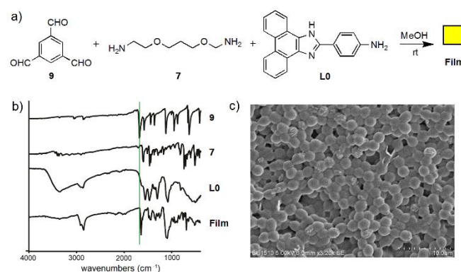
Figure 4. a) Preparation of the fluorodynamic film from trialdehyde 9 , diamine linker 7 and fluorescent amine L0 ; b) Infrared (IR) spectroscopy of the film compared to individual starting components; c) Scanning electron microscopy (SEM) image of the film surface.
