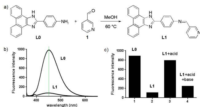
Figure 2. a) Imine formation reaction from fluorescent amine L0 and aldehyde 1 ; b) fluorescent spectroscopy of L0 and L1 (under \lambda_{\text{ex}} 350 nm); c) the fluorescent intensity changes of L1 subjected to acid and base treatments.
