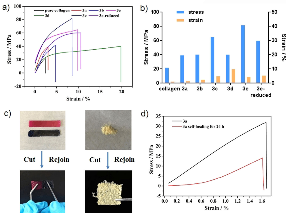
Figure 1. a) Tensile stress-strain curves collagen C, dynameric collagen 3a–e membranes and reduced 3e membrane. b) The highest tensile stress and break strain for each membrane. c) Cutting and rejoining of the self-healing membranes. d) Stress-strain curves of the original and the re-healed membrane 3a .
