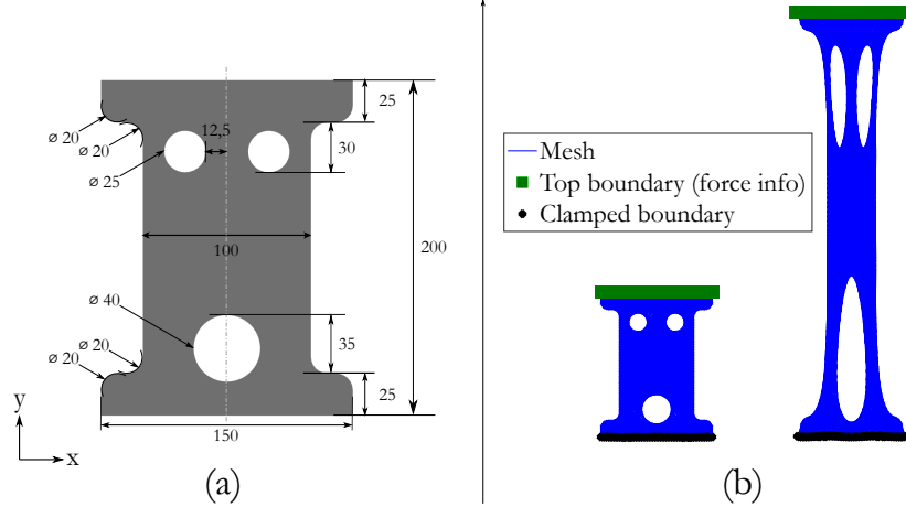
Figure 3: Case of study: a perforated hyperelastic membrane under uniaxial tension ( (a): initial mesh; (b): after 200% of total macroscopic strain). On the top nodes, information on force is available while the bottom ones are clamped.
