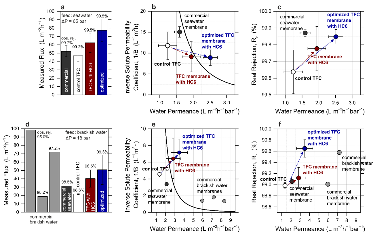
Fig. 3 | Performance of the membranes in the desalination of (a-c) seawater and (d-f) brackish water. (a, d) Experimental water flux and observed solute rejection of control TFC membranes, commercial membranes, and TFC-HC6 membranes incorporating AWCs at 0% recovery. The filtration conditions were: 65 bar applied pressure with 35000 ppm NaCl feed solution at pH 8 for seawater desalination; 18 bar applied pressure with 5800 ppm NaCl feed solution at pH 7 for brackish water desalination. (b, e) Selectivity-productivity trade-off graphs plotting the inverse solute permeability coefficient of the membranes as a function of their respective water permeance; the solid line depicts the proposed TFC upper bound relationship. (c, f) Calculated real rejection of the membranes as a function of respective water permeance. The feed solution temperature in all the tests was 27 \pm 1 °C.
