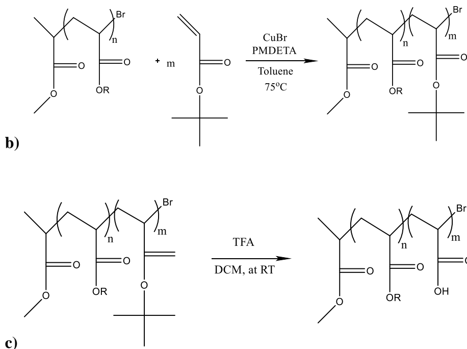
Figure 1 Synthetic steps to prepare the poly(alkylacrylate)-b-poly(acrylic acid) block copolymers by the ATRP procedure. a) polymerization of the alkylacrylate block; b) polymerization of the t-butyl acrylate block; intermediate product; c) hydrolysis of the intermediate product to yield the final product
