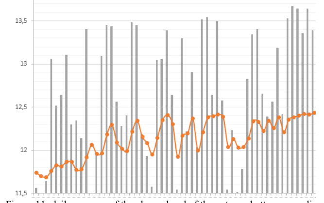
Figure 11: daily average of the charge level of the antenna battery according to the sunshine (gray)
