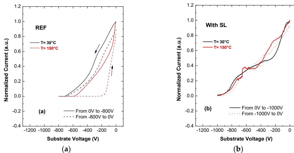
Figure 7. Substrate ramp measurements at room and high temperature. (a) Sample without SL, substrate voltage from 0 V to -800\text{ V} and (b) sample with SL, substrate voltage from 0 V to -1000\text{ V} .
