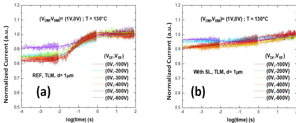
Figure 8. Back-gating transient at T = 130^\circ C on TLM with distance of 1 \mu m under six trapping conditions, (a) Sample A, reference device without SL, (b) Sample B, device with SL.
