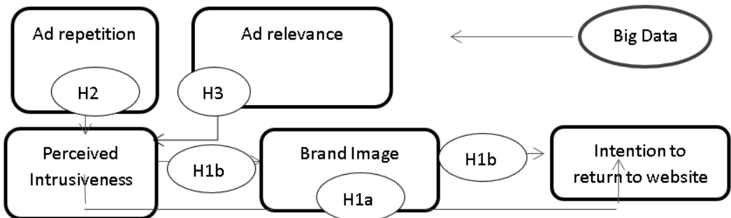
Figure 1: conceptual model
