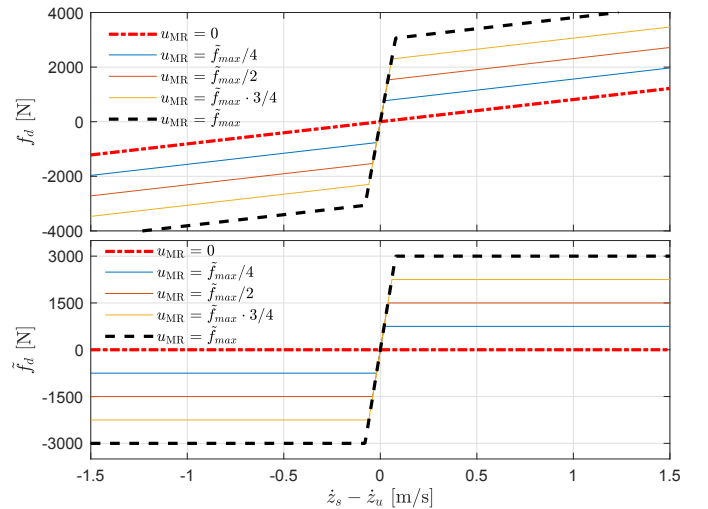
Fig. 1. Typical force-speed curve associated to a MR suspension (upper plot) and the corresponding nonlinearity (lower plot).
