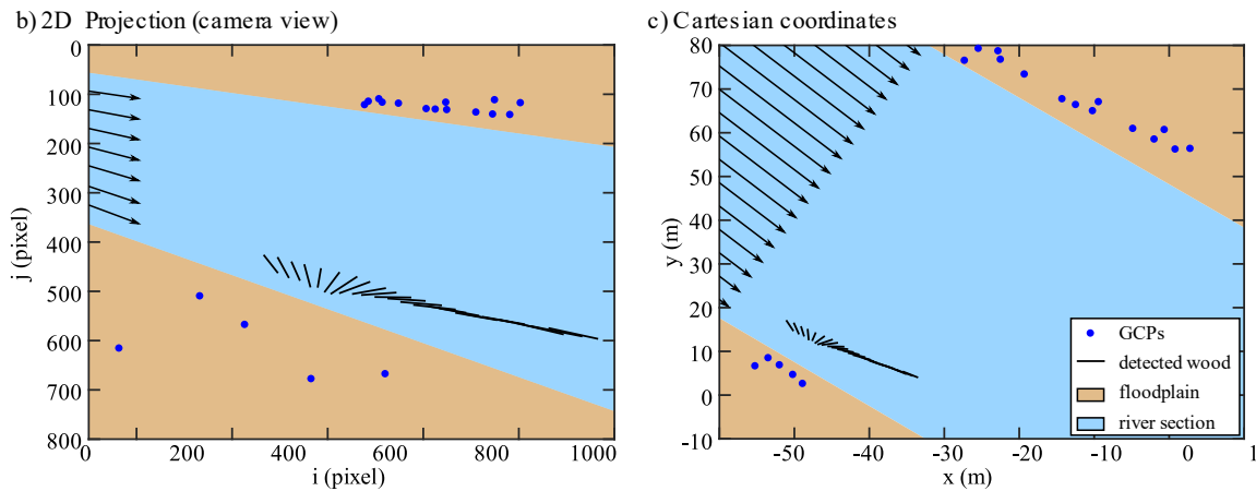
Fig 5 Image rectification, process. 3D view of non-collinear GCPs in metric coordinates (a), their corresponding localization within the image (b), and the relative 2D metric coordinates for a given water level (c). (b,c) A practical example of the transformation of the coordinates is presented. The different solid lines represent the successive detection in a set of consecutive frames.
