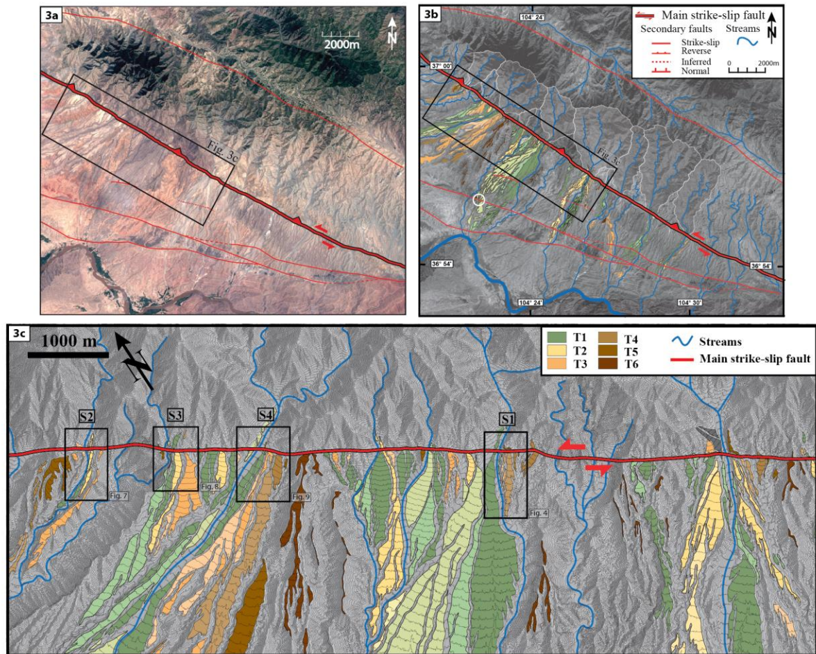
Figure 3: a) Multispectral Pleiades satellite image of studied fault segment. b) Morphotectonic map of Hasi Shan fault segment based on panchromatic Pleiades image (0.5 m resolution). Catchment areas are outlined in white. Colored patches are alluvial and fan surfaces. White circle shows location of offset along secondary fault. Black rectangle is location of figure 3c. c) Enlarged morphotectonic map based on high resolution DEM computed from tri-stereo Pleiades images. Contour lines every 10 m. Black rectangles are location of sites S1, S2, S3 and S4 and figures 4, 7, 8 and 9, respectively.
