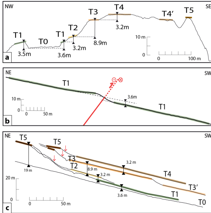
Figure 5: (a) Fault parallel topographic profile at site S1. Color-coding of terraces as in Figure 4. (b) Fault perpendicular topographic profile of T1 on right bank of active stream-bed. (c) Projections of fault perpendicular topographic profiles on left bank of active stream-bed.
