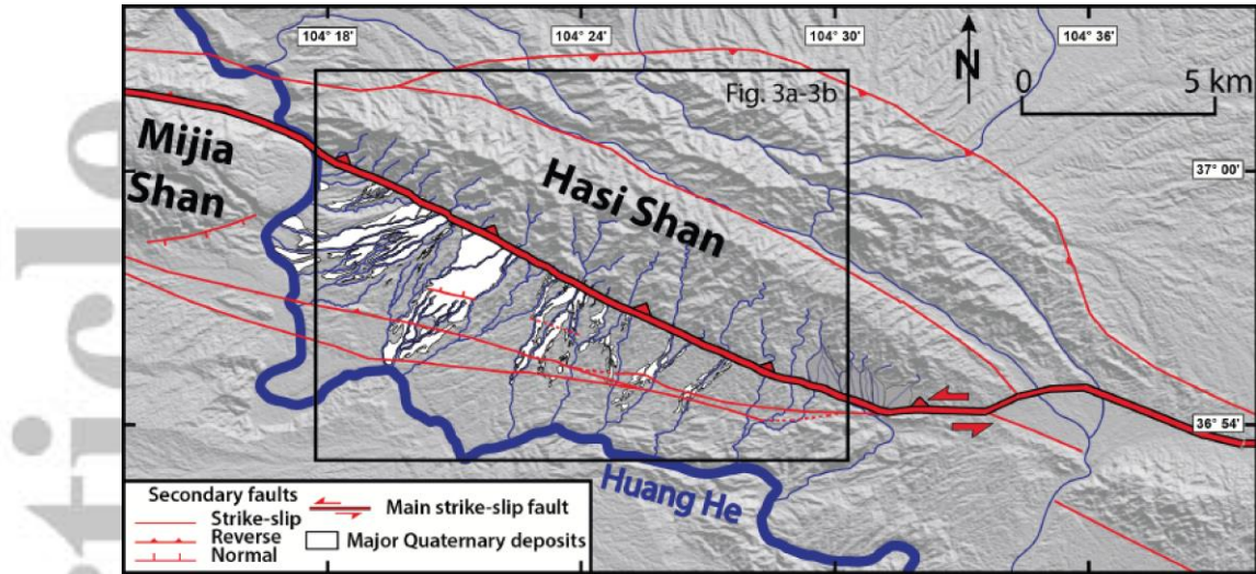
Figure 2: Tectonic setting of Hasi Shan, based on ASTER GDEM. Dissected fan surfaces of southwest Hasi Shan bajada shown in white. Black rectangle is Figure 3.
