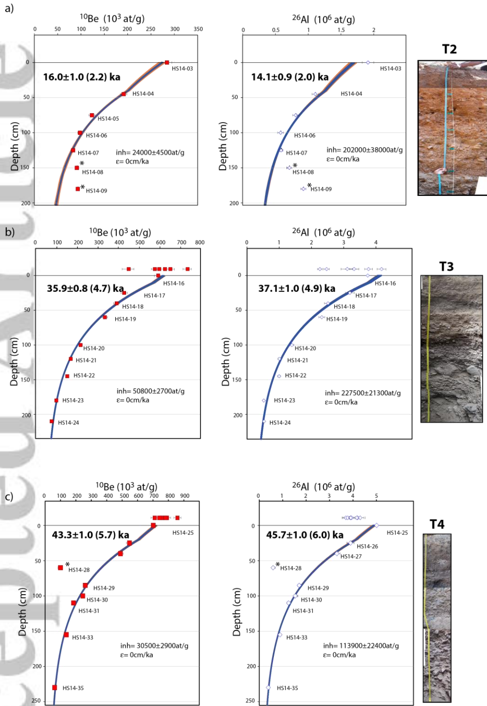
Figure 10: CRN depth profiles derived from gravel and amalgamated samples at site 1 for T2 (a), T3 (b) and T4 (c). Surface sample concentrations are indicated for T3 and T4. ^{10}\text{Be} to the left, ^{26}\text{Al} to the right. A global mean SLHL spallogenic production rate of 4.01 \pm 0.33 at/g/yr for ^{10}\text{Be} (Borchers et al., 2016) and a ^{26}\text{Al}/^{10}\text{Be} spallogenic production ratio of 6.61 (Braucher et al., 2011) are used to scale the local production rates and calculate ages. Model solution are indicated with internal errors (external errors within brackets).
