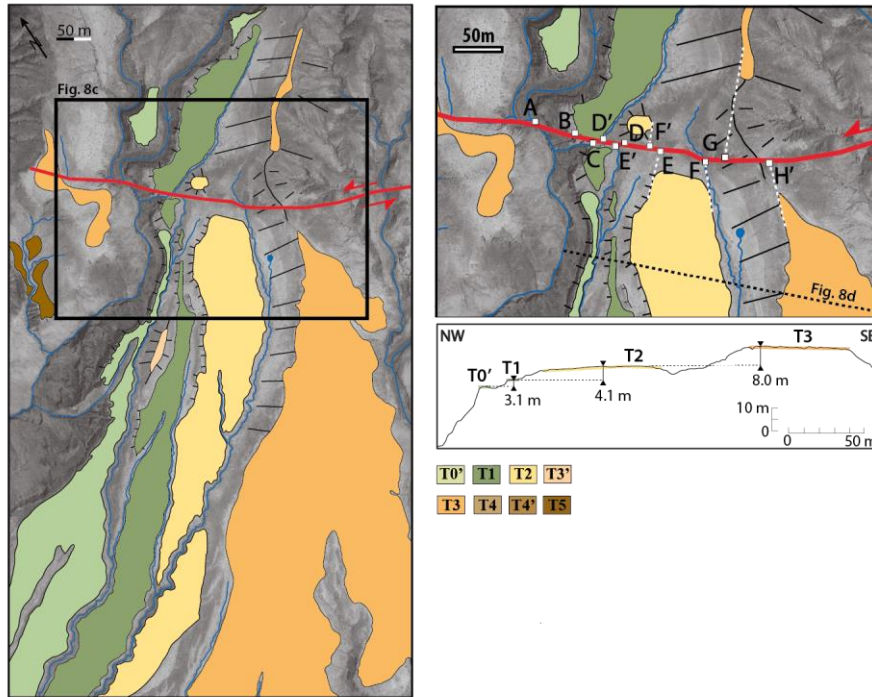
Figure 8: (a) Enlargement of Pleiades image at site S3. (b) Geomorphic interpretation. Black frame outlines location of Figure 8c. (c) Detailed mapping. Dashed black line outlines location of topographic profile in Figure 8d. White squares with letter labels are piercing points, summarized in Table 1 . (d) Fault parallel topographic profile.
