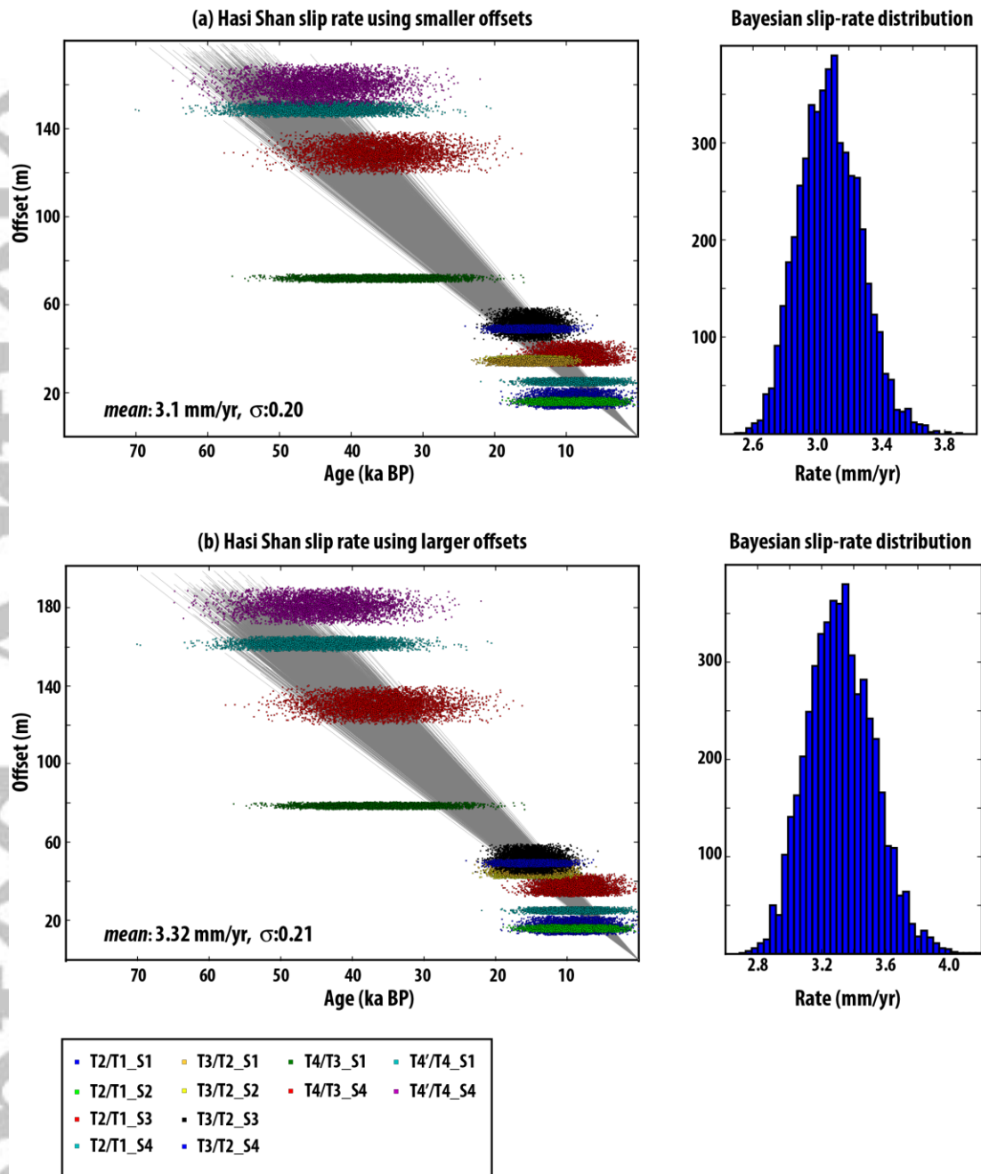
Figure 12: Slip rate estimates using a Bayesian approach [Styron, 2015]. a) and b) show respectively slip rates determined using minimum and maximum offset bounds outlined by piercing lines at sites S1 to S4. Uncertainty for slip-rate is one-sigma (see also Table 1 ).
