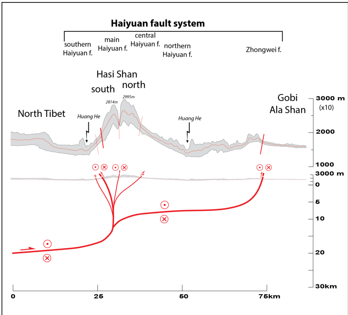
Figure 14: General cross section of entire Haiyuan fault system showing possible fault strands geometry and link at depth (adapted from [Gaudemer et al., 1995; Daout et al., 2016]). Upper panel shows vertical topography exaggerated 10 times.
