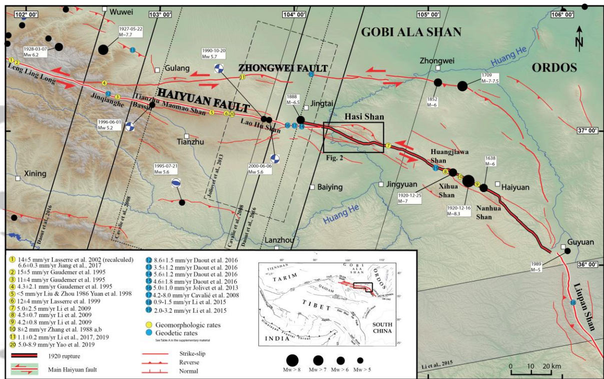
Figure 1: Active faults along Haiyuan fault system. Topography ASTER GDEM (30m resolution; https://lpdaac.usgs.gov/ ). Earthquakes (black dot) and focal mechanisms from USGS. Yellow and blue circles are geomorphic and geodetic slip-rates available in literature (see also Table S1 ), respectively. Dotted, dashed and continuous black rectangles are InSAR swaths. Black rectangle outlines figure 2.
