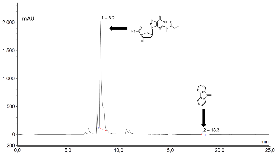
Figure 2.3 Chromatogram of crude deprotection of 3c at 260 nm. t_R (product) = 8.2 min, t_R (fluvone) = 18.3 min.
