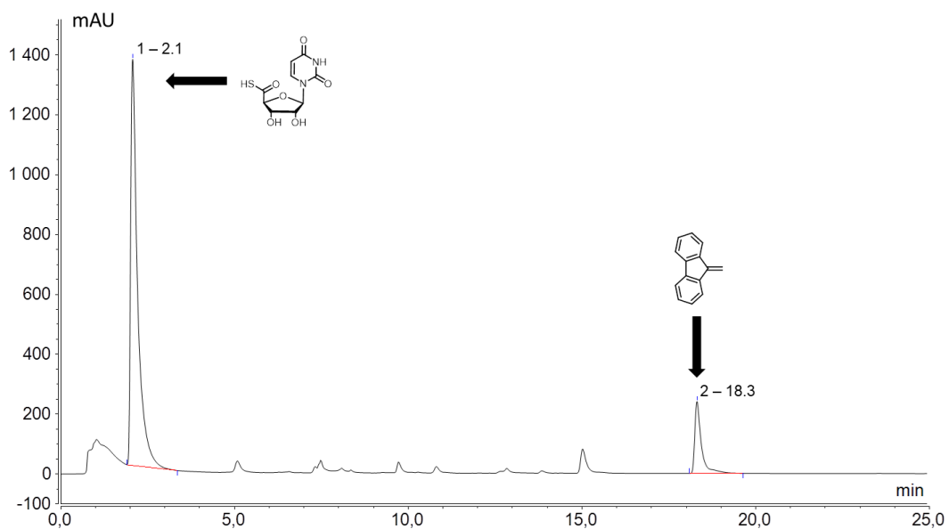
Figure 2.4 Chromatogram of crude deprotection of 3d at 260 nm. t_R (product) = 2.1 min, t_R (fluvone) = 18.3 min.
