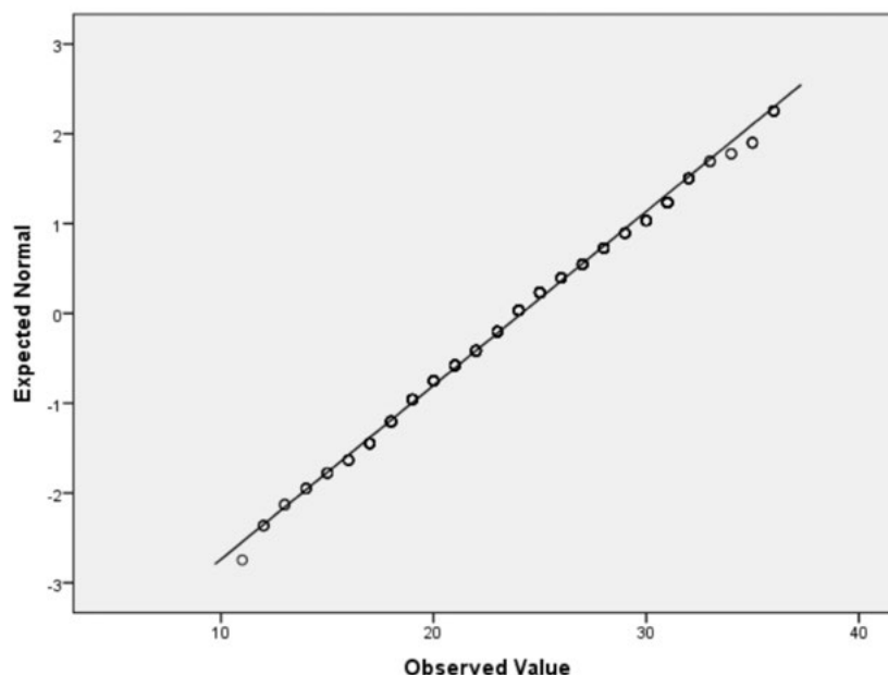
Figure 1 - Normal Q-Q Plot of PSC
