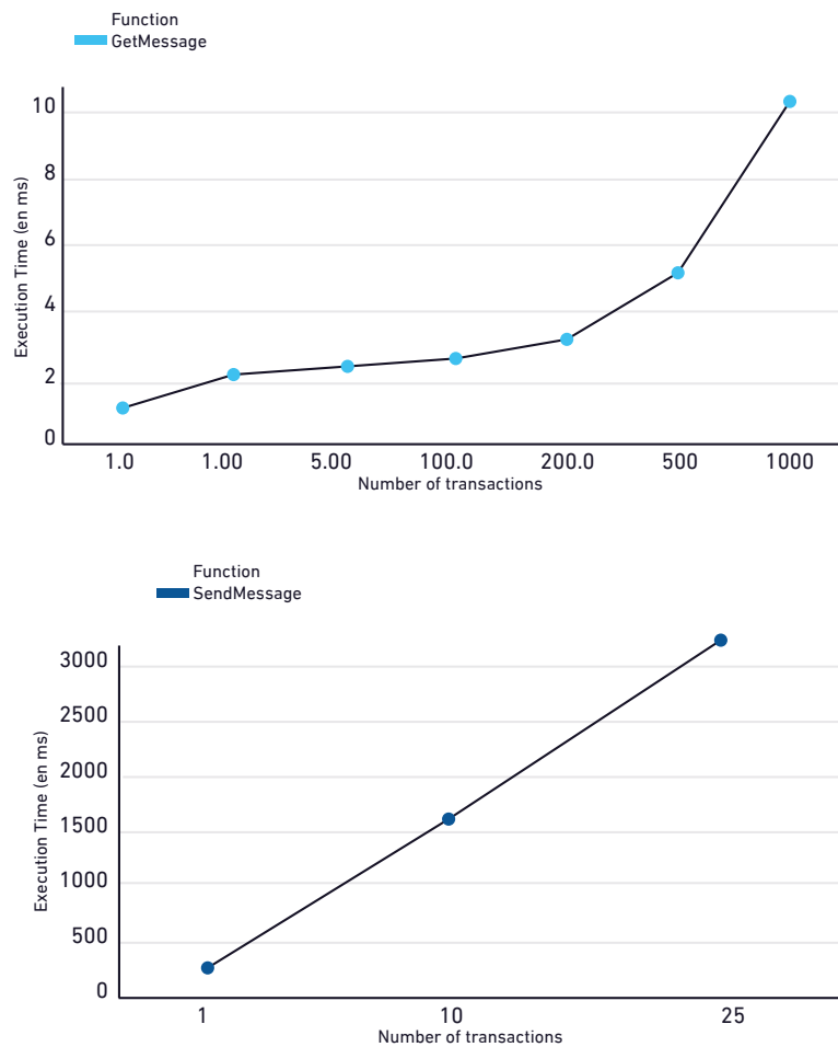
Figure 9. Execution time of the different functions in the Decentralized IoT solution for Vehicles communication (DISV) in milliseconds.
