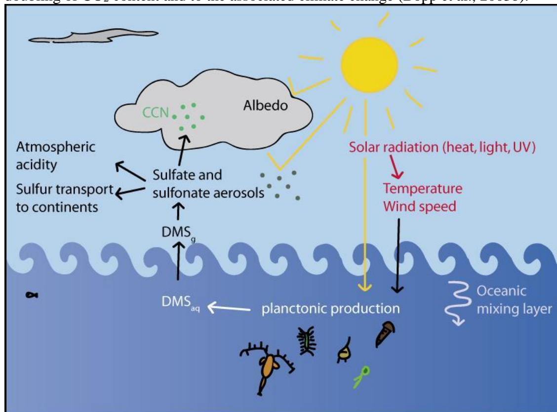
Figure 16 – Feedback mechanisms linking our planet’s climate to DMS emissions from the ocean (adapted from Charlson et al., 1987).
