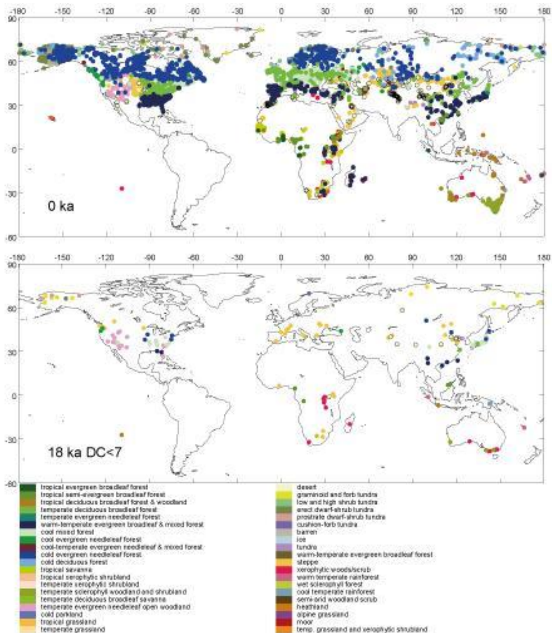
Figure 7. Land vegetation maps for the modern era and the LGM, data from Prentice et al. (2000), Harrison et al. (2001), Bigelow et al. (2003) and Pickett et al. (2004). This figure with homogenised nomenclature has been downloaded from http://www.bridge.bris.ac.uk/resources/Databases/BIOMES_data .
