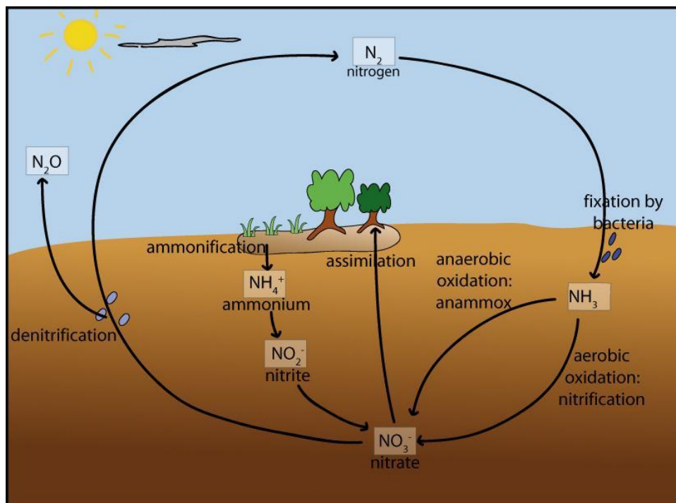
Figure 11. Diagram of the nitrogen cycle
