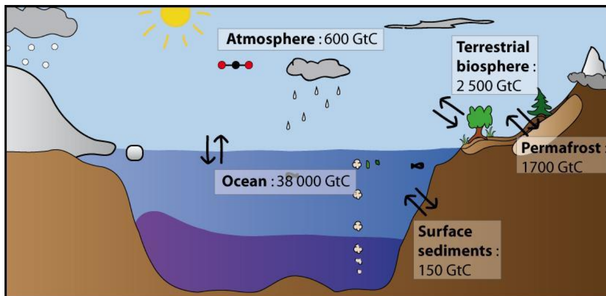
Figure 2. Diagram of the short term carbon cycle (up to a few tens of thousands years).
