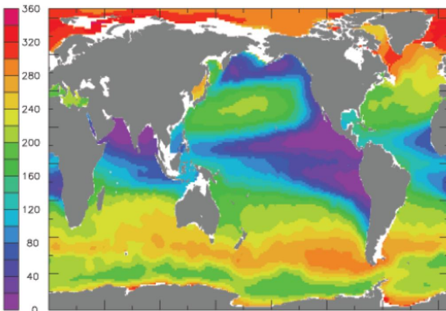
Figure 13. \text{O}_2 concentrations at mid ocean depth (averaged over 200 to 600m, in micromole/L) from the World Ocean Atlas (2009) (Garcia et al., 2010).
