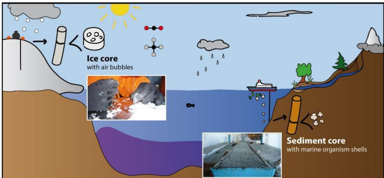
Figure 1. Diagram of the Earth system and schemes showing ice cores and sediment cores extraction.
