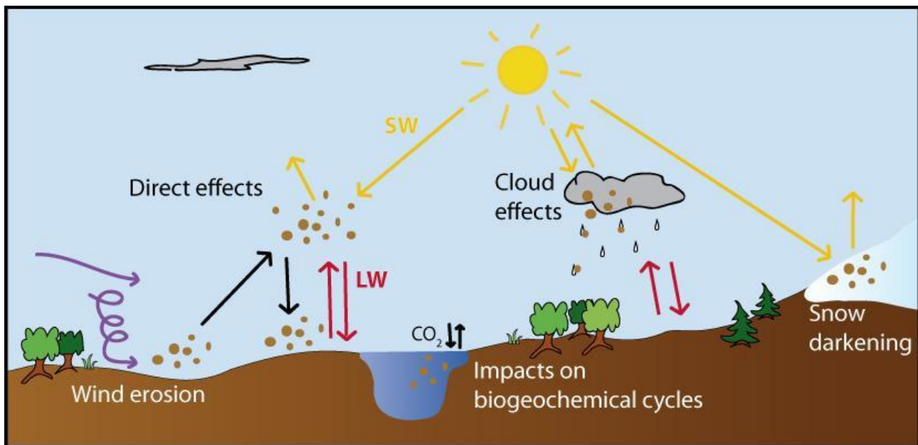
Figure 17. Overview of the dust cycle and its interactions with the climate system.
