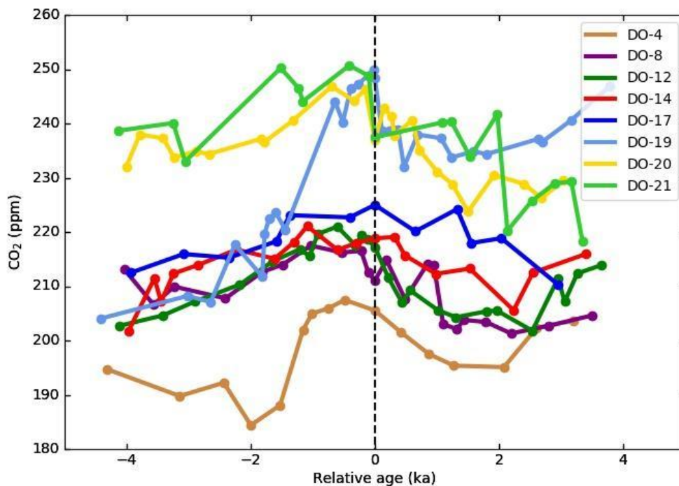
Figure 9. CO 2 variations relative to abrupt warming in Greenland as presented in Ahn and Brook (2008).
