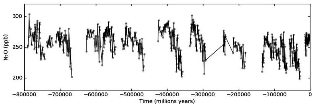
Figure 12. Evolution of \text{N}_2\text{O} (ppb), over the last 800 000 years. Data from Schilt et al., (2010).
