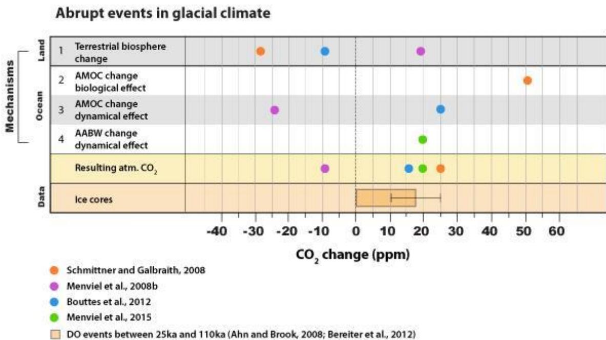
Figure 10. Changes of atmospheric CO 2 due to different processes in atmosphere-ocean-terrestrial biosphere model simulations with glacial background climate. Figure modified from Mariotti et al., 2013. Model data are taken from the simulations with maximum CO 2 change and at the time when atmospheric CO 2 for ocean and land carbon changes is at a peak.
