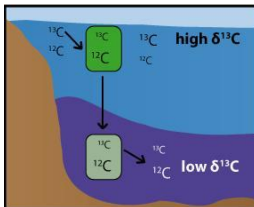
Figure 6. Diagram of \delta^{13}\text{C} in the surface and deep ocean. In the surface waters, the value of oceanic \delta^{13}\text{C} is high because of photosynthetic activity, which preferentially uses light ^{12}\text{C} , thus enriching the environment with heavy ^{13}\text{C} . In the deep ocean, remineralisation releases carbon with more ^{12}\text{C} , therefore lowering \delta^{13}\text{C} .
