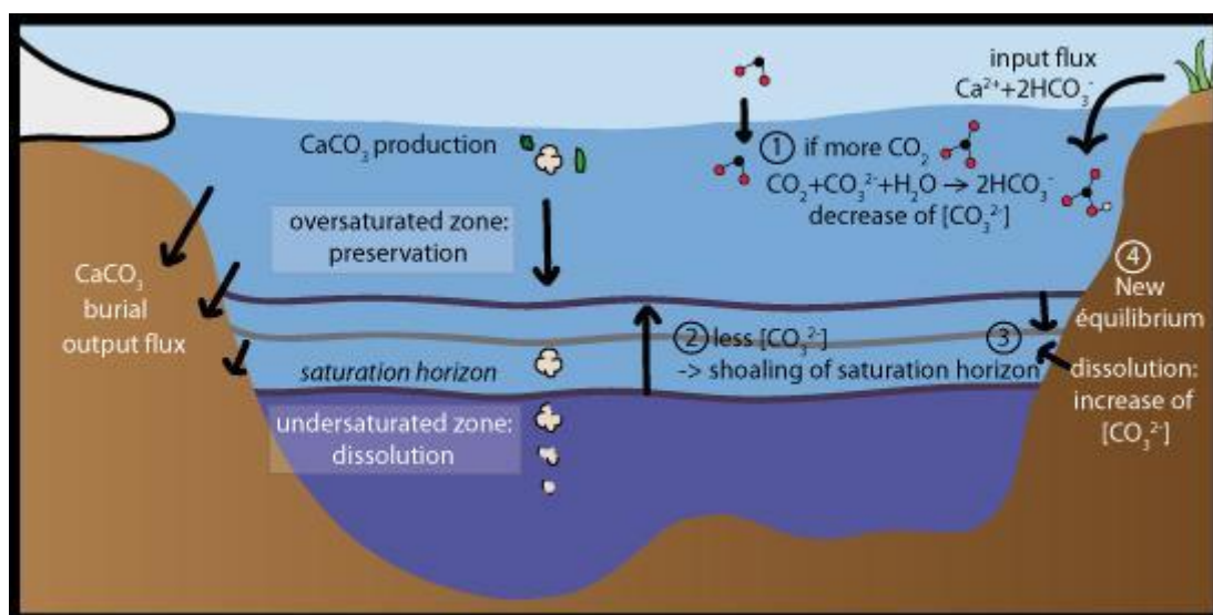
Figure 8. Diagram of the carbonate compensation mechanism.
