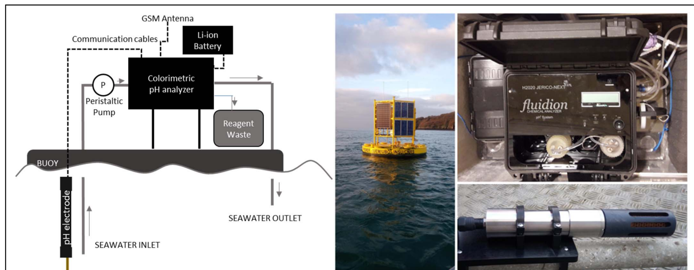
Fig. 2. Schematic (left) and photo (right) of the surface buoy hybrid system. The photo shows the hybrid pH system on the MAREL-Iroise buoy in January 2019. Left: MAREL-Iroise buoy. Top right: analyzer and battery in the aluminum box on the buoy. Bottom right: pH electrode on the aluminum pole ready to be deployed.
