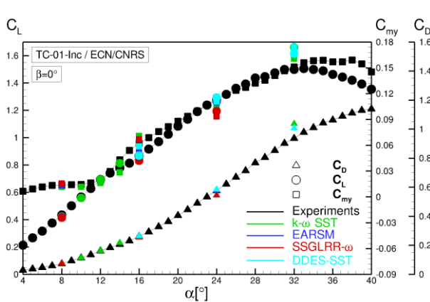
Figure 5. Comparison of aerodynamic coefficients, drag coefficient, lift coefficient and pitching moment coefficient, versus the angle of attack \alpha
