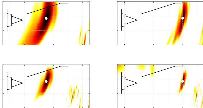
Figure 3: Point Spread Functions at M=0.85 for sources at two different normalized frequencies (top: 1.66, bottom: 3.33) and two different positions (left/right). Source positions are materialized by white dots. Color scale dynamic 20dB.
