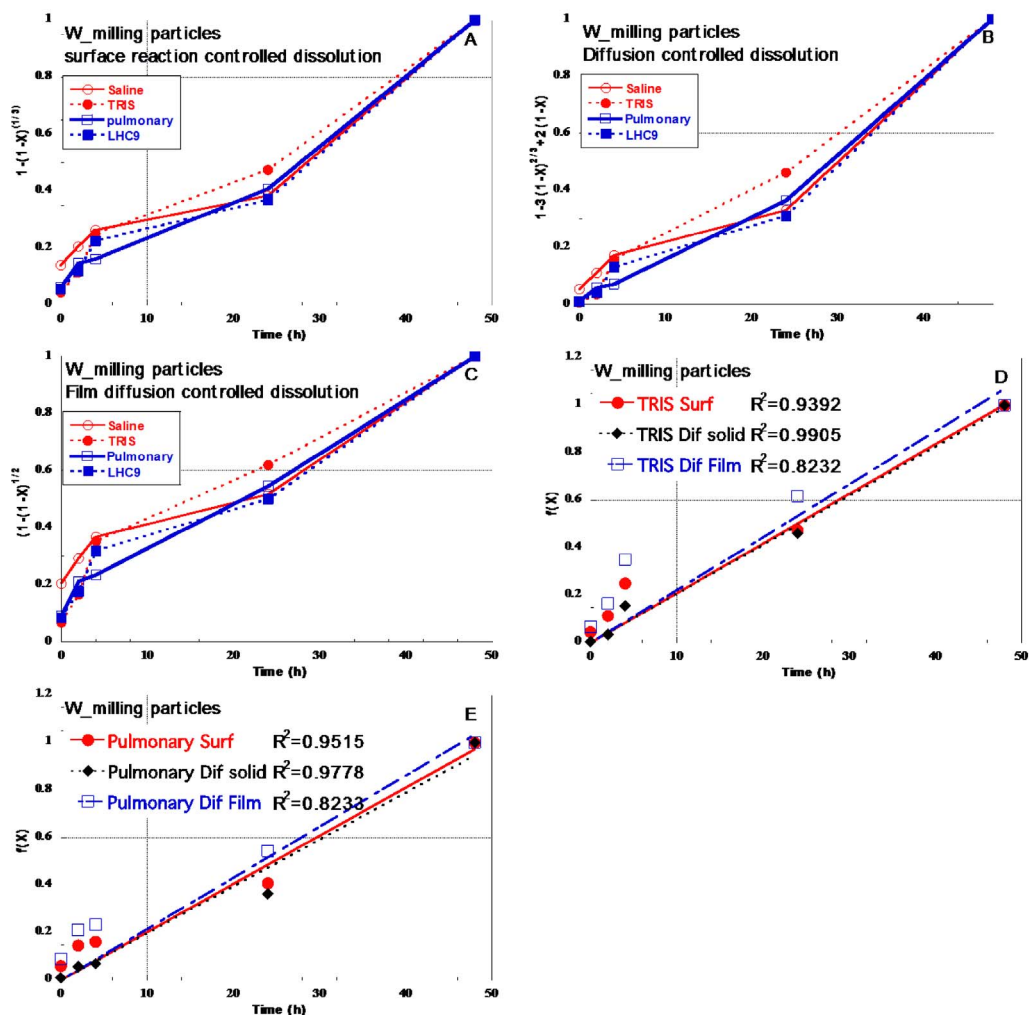
Figure 9. Assessment of (1), (2) and (3), which correspond to the different controlling stages of the shrinking core model. In the plots, the slope represents k_{\text{exp}} .
